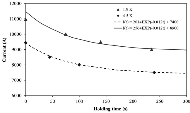
Fig. 10. Quench current at current plateau vs. holding time at 4.5 K and 1.9 K.
