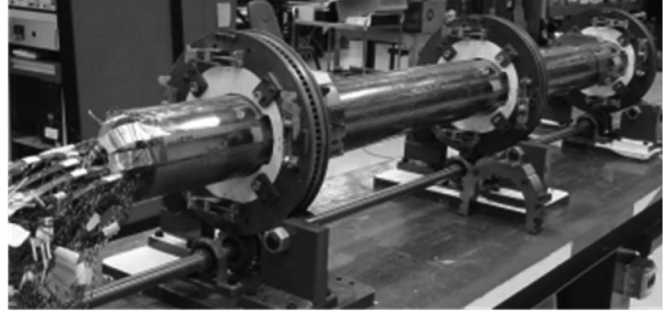
Fig. 4. Assembly of two dipole coils with protection heaters and ground insulation.
