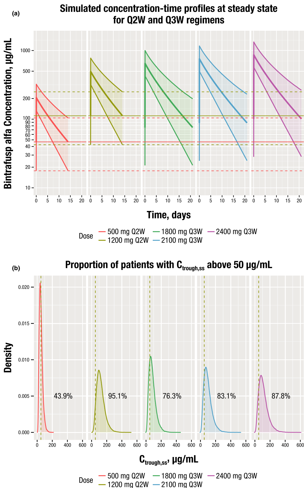
Figure 4 Simulated concentration-time profiles at steady state for q2w and q3w regimens (a) and proportions of patients above the target trough concentration ( C_{\text{trough}} ) of 50 µg/mL at steady state (b). Lines are medians. Shaded areas are 95% prediction intervals. Solid horizontal lines are median steady-state troughs for 500 mg q2w (orange) and 1,200 mg q2w (olive). Dashed horizontal lines are the 95% predicted range for steady-state troughs for 500 mg q2w (orange) and 1,200 mg q2w (olive).
