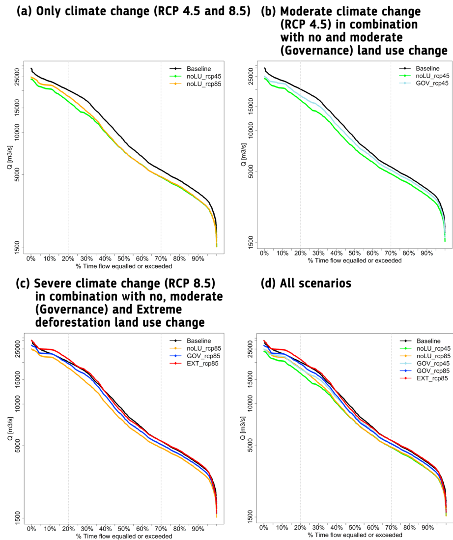
Figure 9. (a–d) Flow duration curve of the baseline (1986–2005) and future (2026–2045) climate and land use scenarios at Itaituba. Flow ( \text{m}^3/\text{s} ) is shown on the y axis and percentage of the time of exceedance of the specific threshold on the x axis. Baseline scenario in black, no land use and moderate climate change (noLU_rcp45) in green, no land use and severe climate change (noLU_rcp85) in orange, moderate land use (Governance) and climate change (GOV_rcp45) in light blue, moderate land use (Governance) and severe climate change (GOV_rcp85) in dark blue, and severe land use (Extreme) and severe climate change (EXT_rcp85) in red. RCP = Representative Concentration Pathway.
