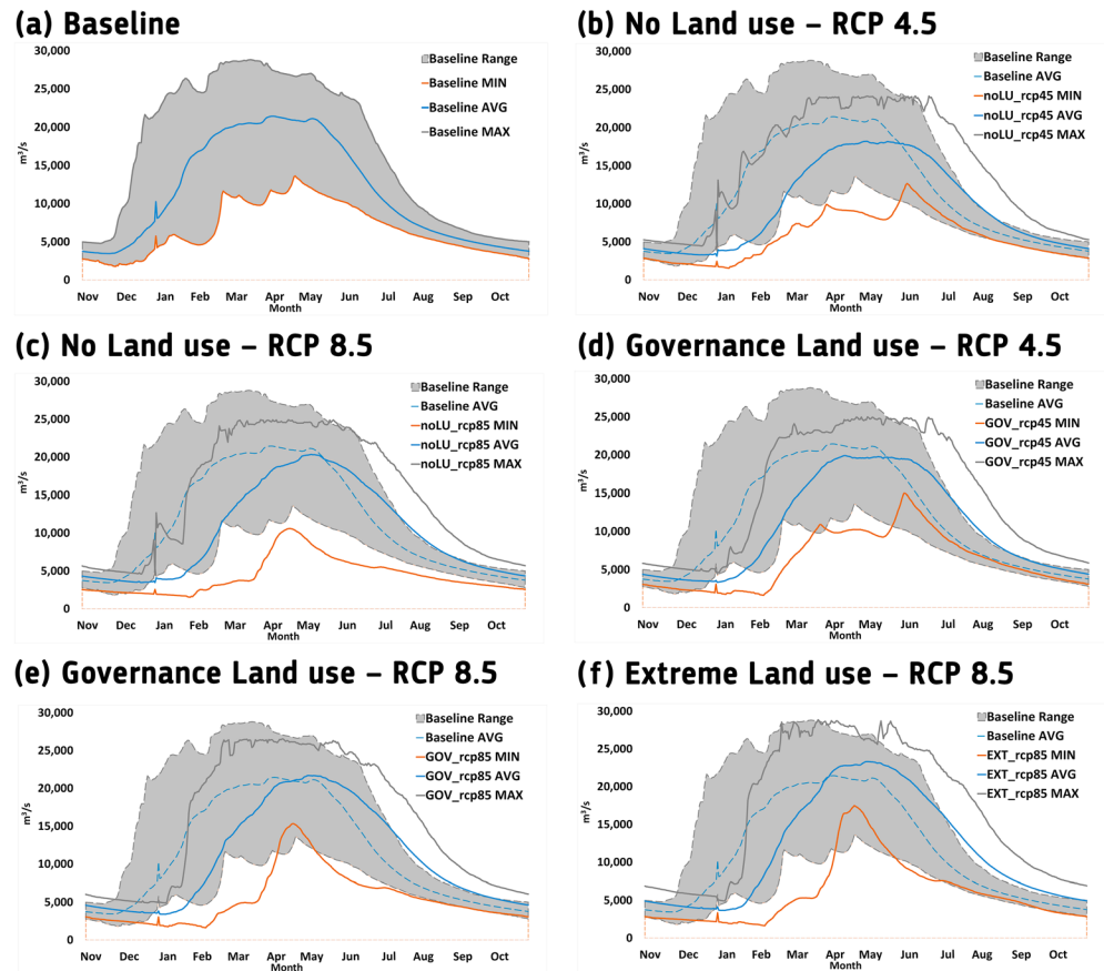
Figure 11. (a) Average, minimum, and maximum daily flow values for the baseline (1986–2005) and future (2026–2045) climate and land use change scenarios at Itaituba. On the y axis flow ( m^3/s ), on the x axis time (from November to October). In panels (b) to (f), the blue dashed lines represent the baseline average, minimum, and maximum and the gray shaded area the baseline variability as represented in panel (a). RCP = Representative Concentration Pathway.
