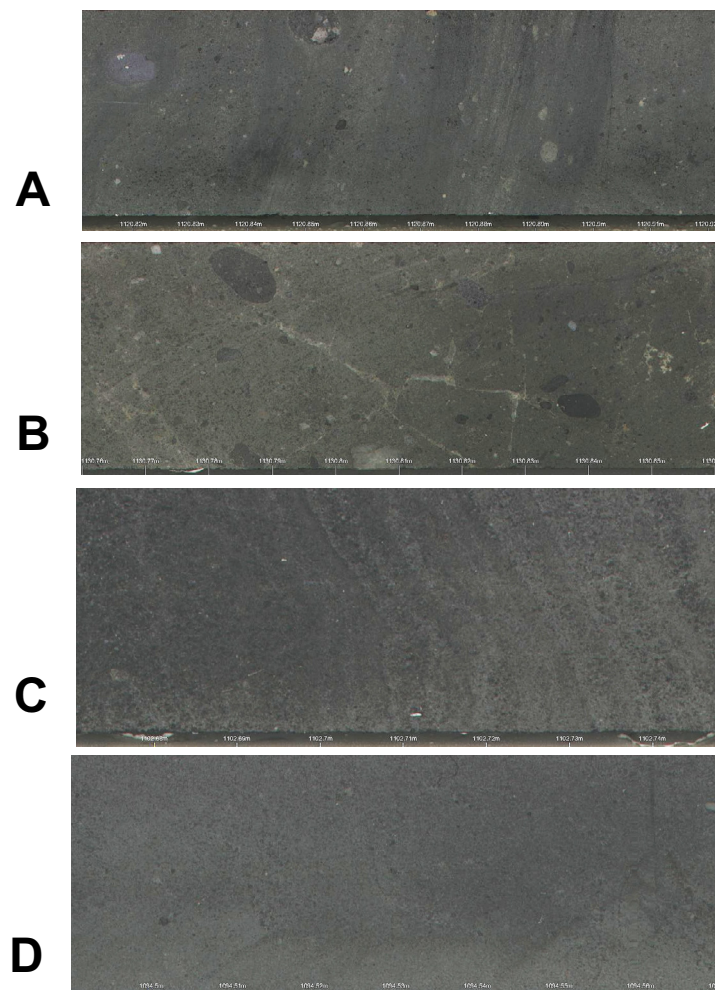
Figure 6. Composite Sequence 1 lithologies showing (A) stratified diamictite, (B) boxwork fractures, (C) laminated sandstone within a sandy interbed, (D) sandy mudstone with coarse sand grains.
