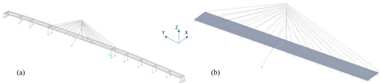
Fig. 4. Structural numerical models: (a) full bridge model; (b) simplified model for cable-stayed span..
