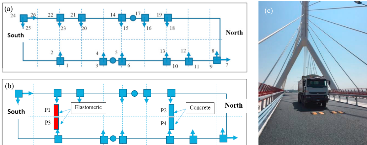
Fig. 1. (a) Accelerometers, and (b) bumpers location on the bridge. (c) 38t truck in the elastomeric bumpers of position P1.
