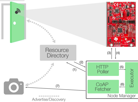
Figure 2: IoT-based surveillance infrastructure.
