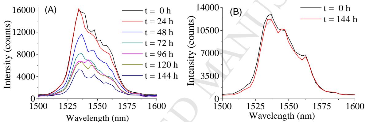
Figure 7. A) Reflected spectra of an OFS embedded in the epoxy exposed to simulated sea water at 80°C. Spectra were collected every 5 min, but only the relevant curves are reported here. B) Reflected spectra of a Cu-OFS embedded in the epoxy exposed to simulated sea water at 80°C.
