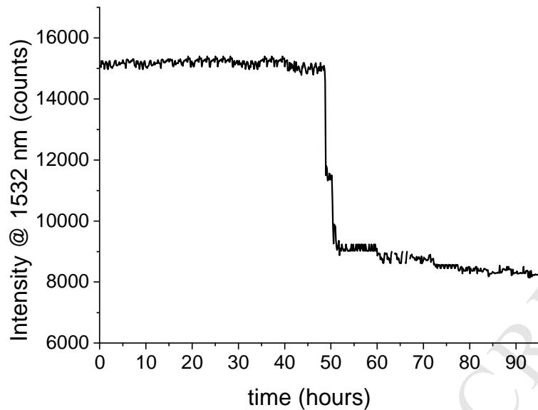
Figure 9. Example of signal recorded from a sensor embedded into an epoxy sample at depth 2.6 mm. The signal drop occurs after a 49 hours exposure of the sample to salty water diffusion (accelerated test at 80 °C). The diffusion length expected from eq. 2 is 2.5 mm.
