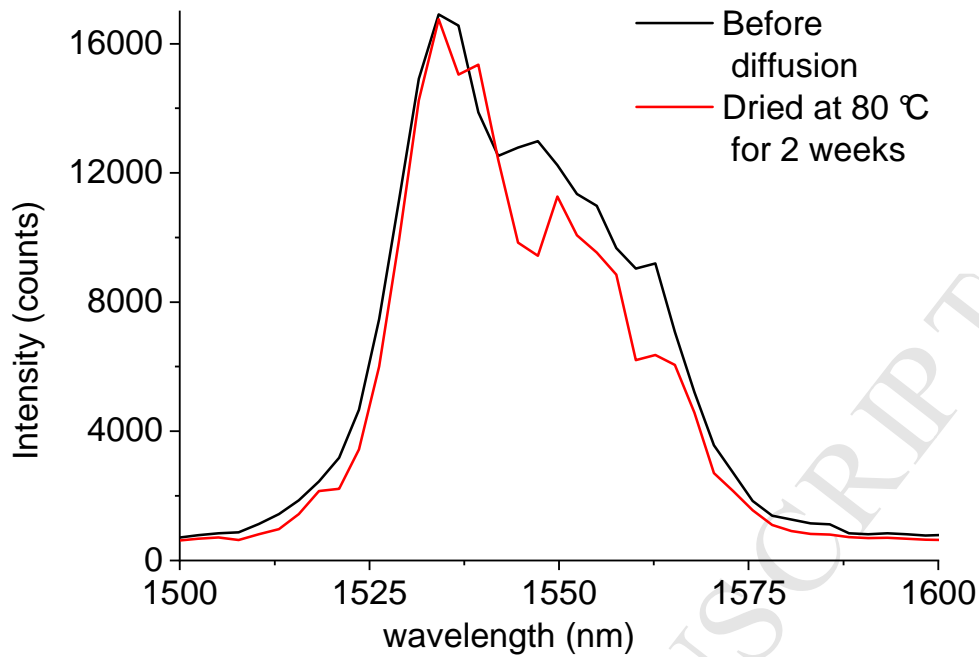
Figure 8. Reflected spectrum before water diffusion (black) and after the water-diffused sample was dried at 80°C for two weeks (red).
