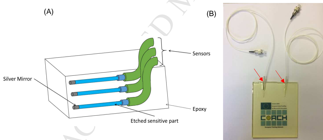
Figure 1. A) Schematic of an epoxy sample with multiple optical fibre sensors (OFSs) with silver (Ag) coated tips embedded at different depths. B) Snapshot of a sample with two embedded OFSs pigtailed to standard telecommunication connectors. The red arrows indicate the protective sleeves.
