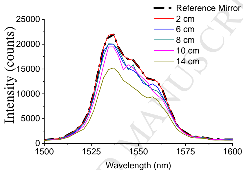
Figure 5. Experimental optimization of the length of the optical fibre sensors obtained from a comparison of the back-reflected spectrum with that of a reference fibre mirror.
