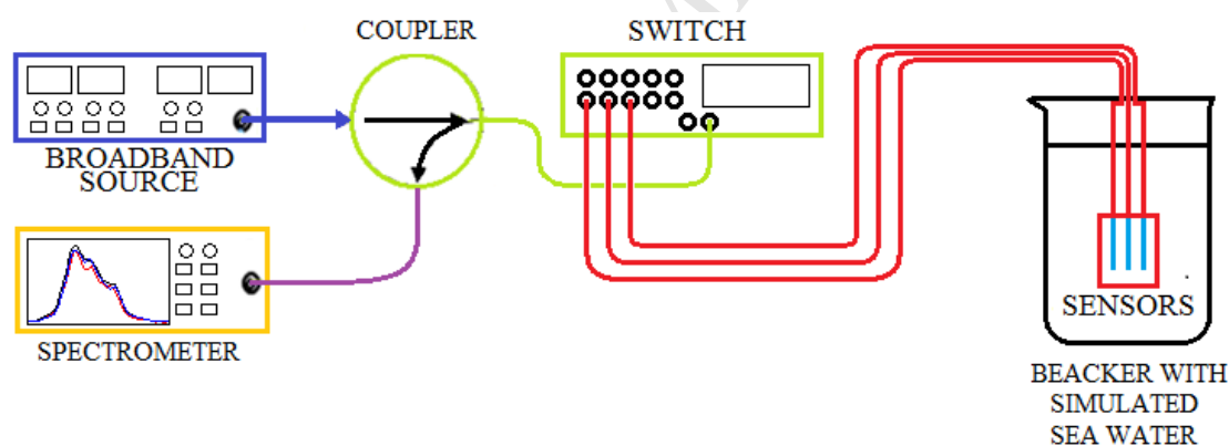
Figure 2. Schematic of the interrogation set up.
