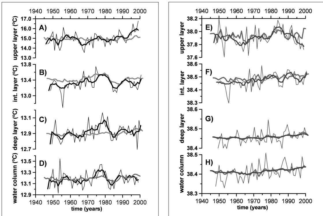
Figs 2A, B, C, D: Temperature evolution for the upper, intermediate, deep layer and integrated water column in the WMED obtained averaging the seven boxes in Fig. 1. Upper layer is considered as 0-200m, the intermediate layer as 200-600m and the deep one as 600m-bottom. Black thin lines are the time series obtained averaging all the MEDATLAS available profiles within each box for each year (non interpolated or averaged raw data in the text). Black thick lines are non interpolated time series smoothed with a five year running mean. Grey thick lines are time series obtained from the interpolated temperature fields averaging the annual profiles from the grid points within the boxes (interpolated time series in the text). Figures 2E, F, G and H are the same for salinity time series.
