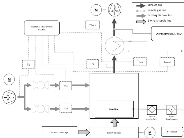
Fig. 2. Control scheme and acquisition lines of the boiler
