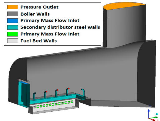
Fig. 3. Boiler boundary conditions overview
