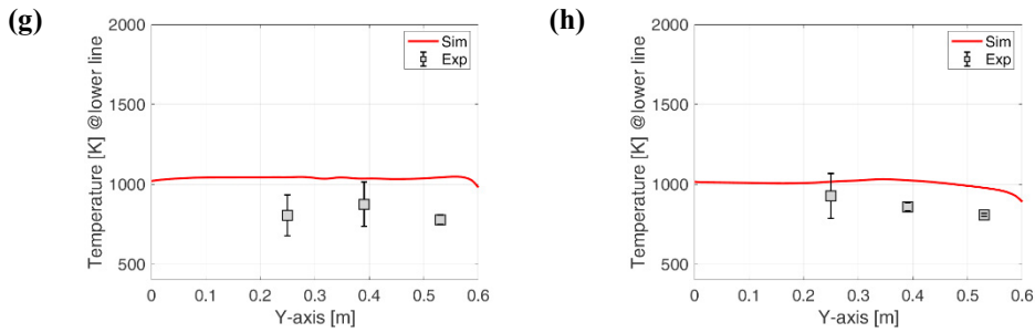
Fig. 4. Experimental (Exp) and predicted (Sim) temperatures in the fixed bed for ID1 (a,c,e,g) and ID2 (b,d,f,h)
