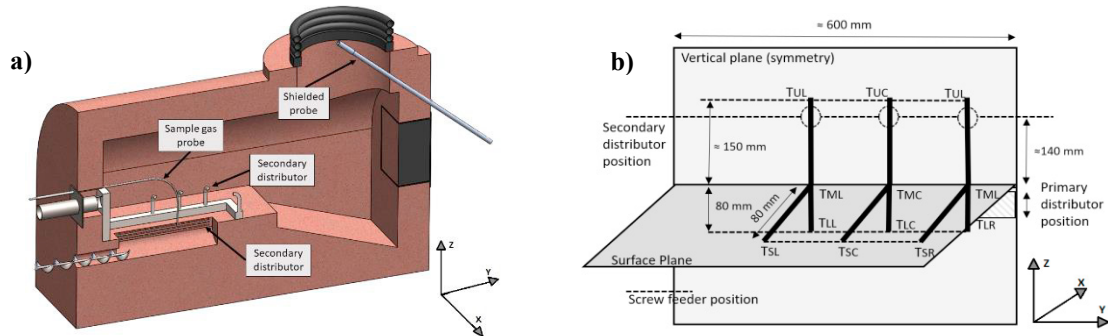
Fig. 1. (a) boiler system overview; (b) thermocouples position scheme
