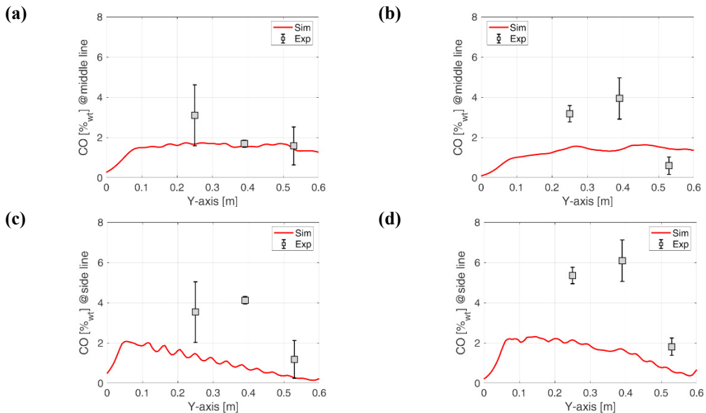
Fig. 5. Experimental (Exp) and Simulated (Sim) CO specie behavior into the fixed bed surface for ID1 (a,c) and ID2 (b,d)
