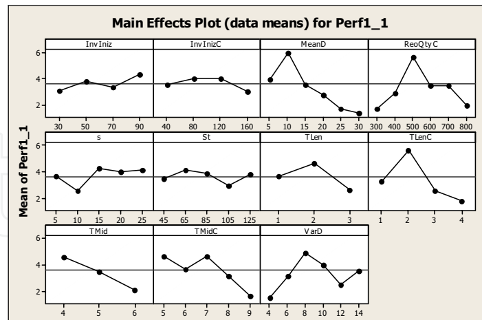
Figure 15. ANOVA Analysis.
