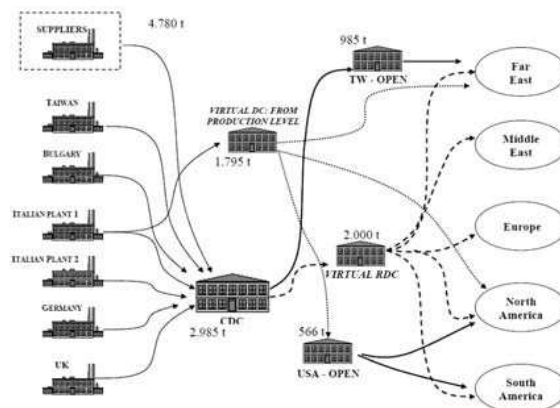
Figure 11. Multi-commodity model
