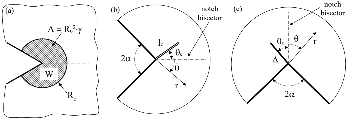
Fig. 1. Reference system for: (a) averaged SED criterion; (b) Leguillon et al. criterion and (c) Carpinteri et al. criterion.
