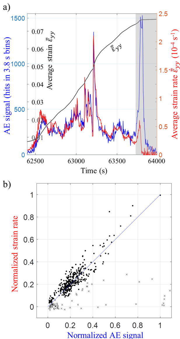
Fig. 3 Concurrent tracking of average-strain and overall AE intermittency during the phase transformation.
