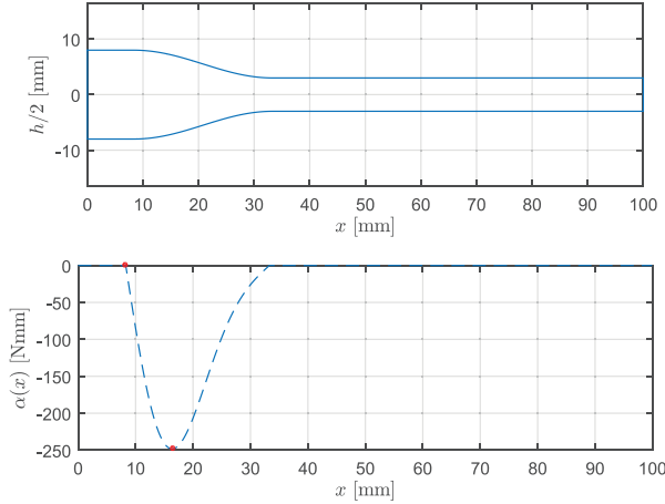
Fig. 20. Body with variable cross section (top), characterized by the negative real part of the SDI. The first derivative of the flexural stiffness is plotted (bottom) and the minimum and the closest maximum are highlighted by red dots.
