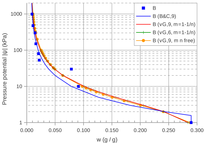
Figure 6. Experimental and interpolated soil-water retention relationships of one of the sandy soils used to repeat Perrault's experiments. B: soil identification; \square : experimental data; B&C: Brooks and Corey's curve; vG: van Genuchten's curve; 6 and 9 are the number of experimental points which were used to interpolate the analytical curves.
