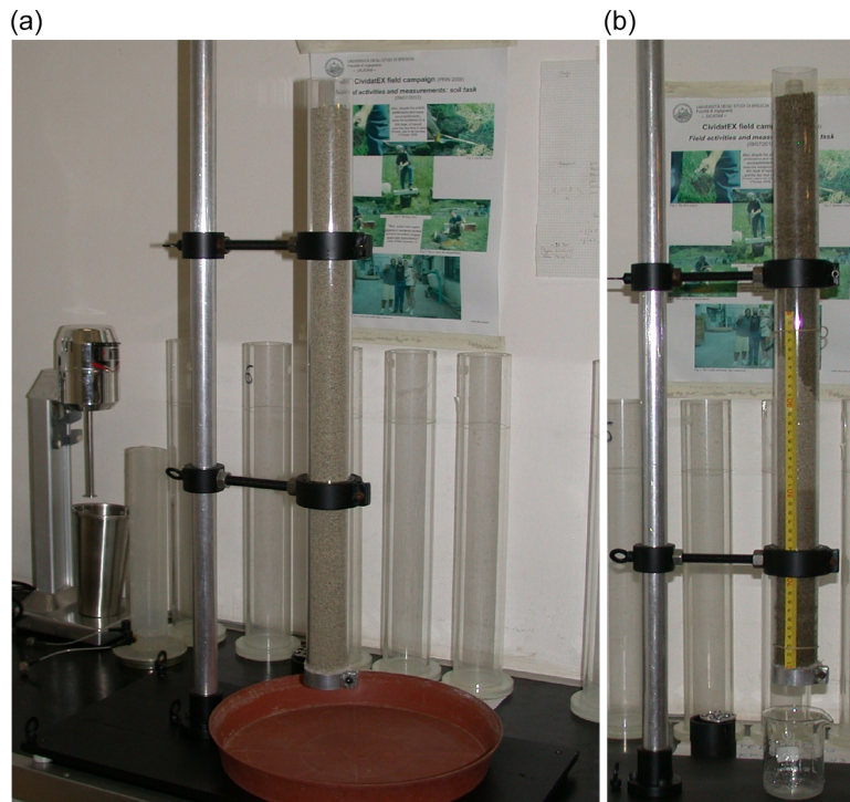
Figure 5. Laboratory setup of the soil column (a) and the soil column during the second part of the first experiment, when the top and the bottom imbibition fronts meet (b).
