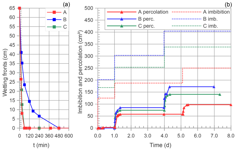
Figure 8. Measures collected during the three repetitions of the third experiment: depth of the imbibition fronts (a) and volumes of imbibition and percolation (b). The unitary volume V_i of a vial was estimated to be equal to V_i = 31.3, 50.5 and 41.0\text{cm}^3 for soil A, B and C, respectively, according to the procedure described in Sect. 5. A, B, C: soil identification; \square : downward moving water front; \triangle : percolation volume; dashed line: imbibition volume.
