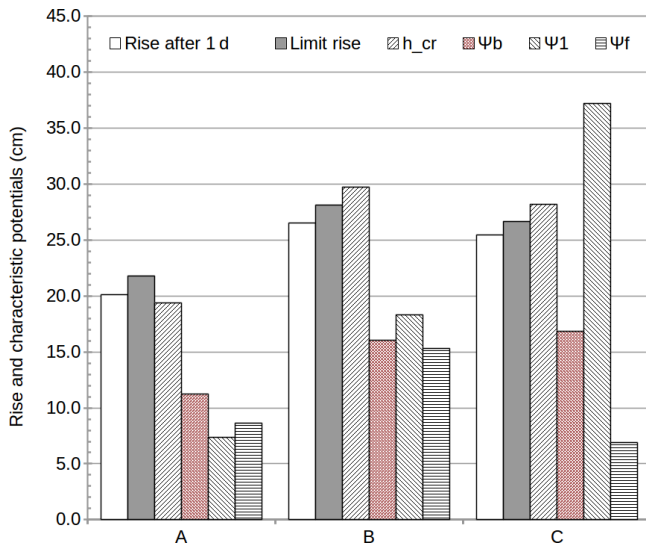
Figure 10. Comparison between the measured height of capillary rise after 1 d, the limit height of capillary rise, the height of capillary rise h_{cr} estimated by means of the Polubarinova-Kochina formula, and the absolute values of the characteristic potentials \Psi_b , \Psi_1 and \Psi_f for the three soils used to repeat Perrault's experiments.
