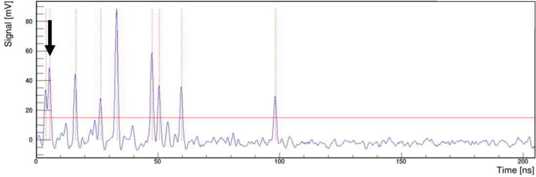
Figure 2. Example of a 200 ns time window collected with the digitizer. The arrow points at a peak with pile-up effect, while the solid red line indicates the chosen threshold to count the peaks produced by incoming particles.
