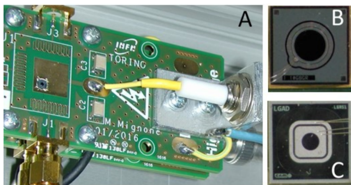
Figure 1. A. Picture of the two sensors mounted in a metallic box and aligned to the beam. B. Hamamatsu sensor ( 1\ \text{mm}\ \varnothing \times 50\ \mu\text{m} thickness). C. CNM sensor ( 1,2 \times 1,2\ \text{mm}^2 \times 50\ \mu\text{m} thickness).
