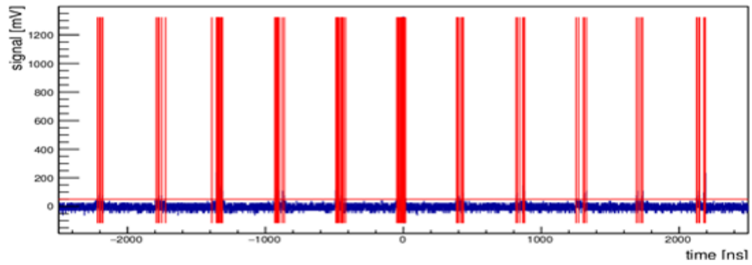
Figure 6. A \mu\text{s} time window of the oscilloscope showing the bunched structure of the CNAO proton beam. The instantaneous fluence inside each bunch is \sim 10^{10} p/s \text{cm}^2 .
