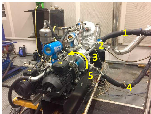
Figure 2. Experimental test bench: 1. Auxiliary suction line; 2. Regulation valve; 3. Aux. suction pressure sensor; 4. Main suction line; 5. Main suction pressure sensor.
