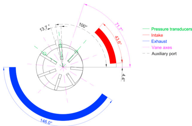
Figure 3. Details of the sliding vane expander.
