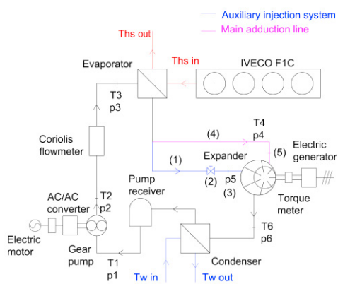
Figure 1. ORC unit scheme.
