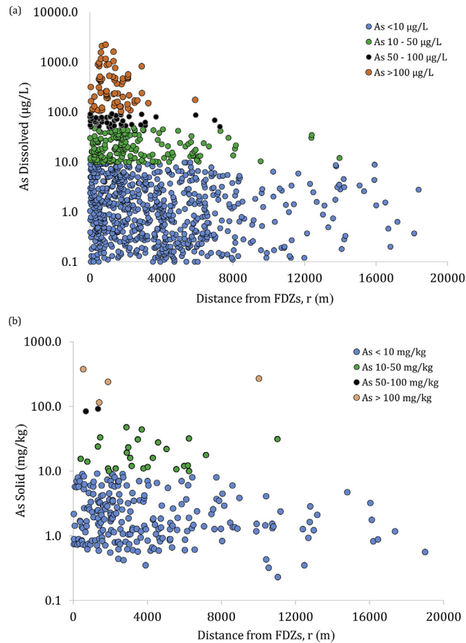
Figure 4. Comparison of concentrations of (a) dissolved As ( \mu\text{g/L} ) and (b) solid phase As ( \text{mg/kg} ) with distance, r (m), from detected fault and deformation zones (FDZs) detected via geological and geophysical surveys, showing the geometrical dependence of As concentrations and major geological features.
