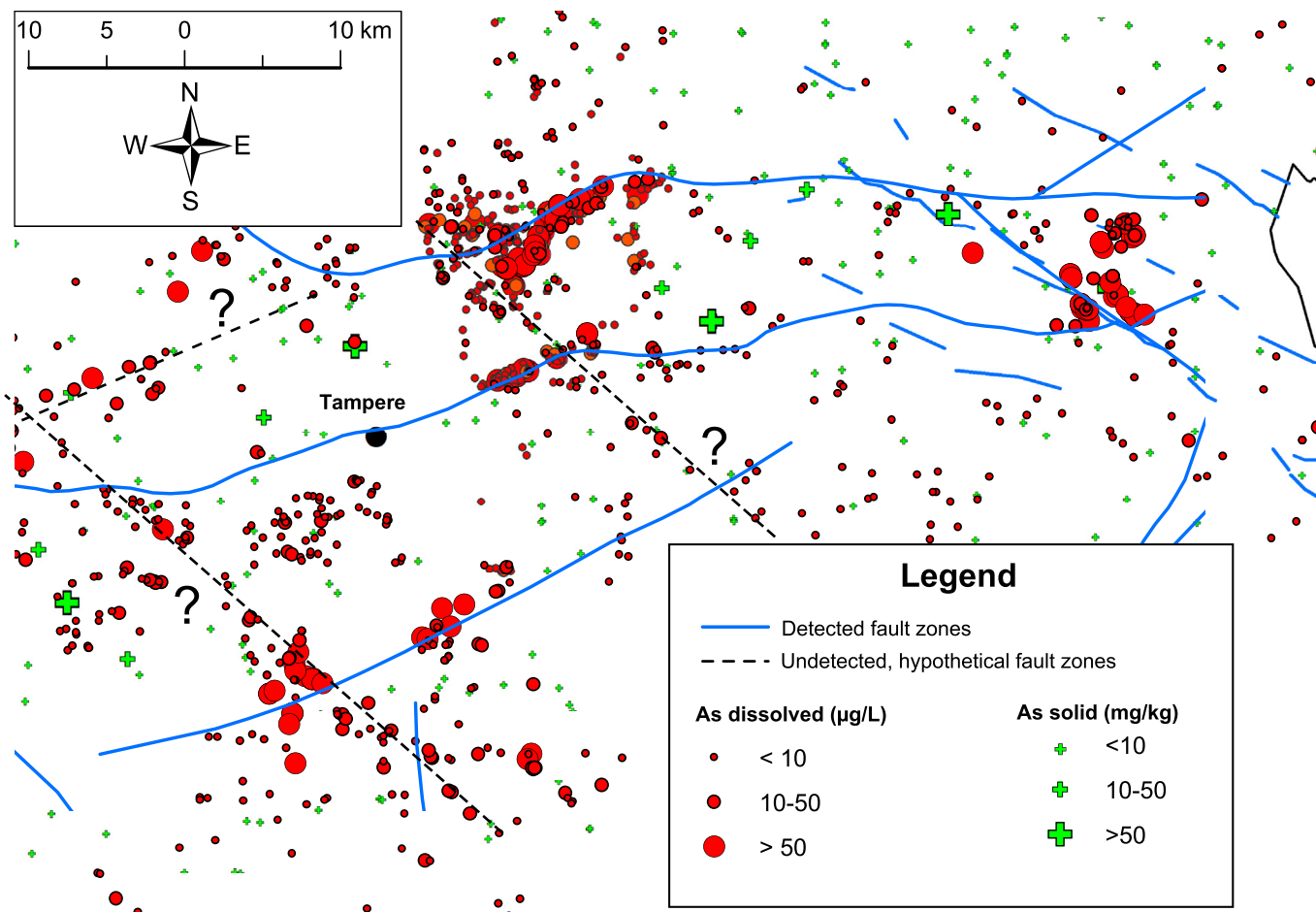
Figure 2. Distribution of dissolved As concentrations ( \mu\text{g/L} ) from samples collected during this study and solid concentrations ( \text{mg/kg} ) in the bedrock reported by Lahtinen (1996) in the southwest Tampere region. Dotted black lines with question marks indicate undetected hypothetical fault and deformation zones (FDZs) in the area inferred from the distribution of high As dissolved concentrations and with orientations similar to the straight blue lines, which represent actual FDZs detected through geological and geophysical surveys (Nironen et al., 2016).
