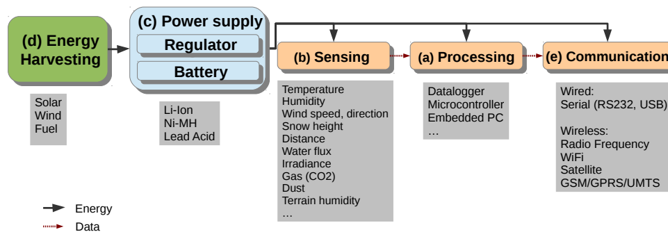
Figure 1. Scheme of typical components of an Automatic Weather Station
