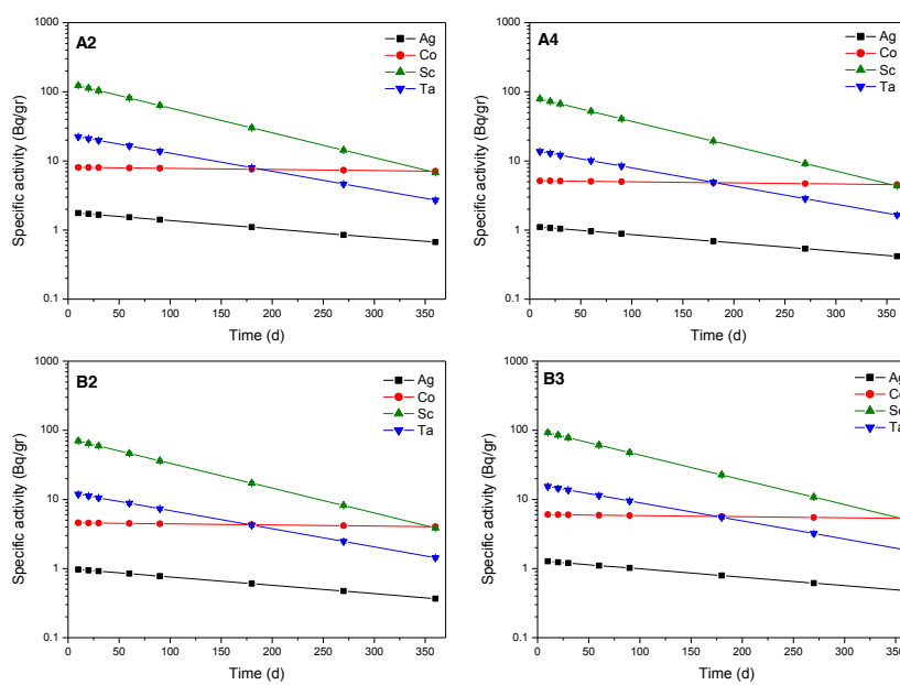
Fig. 4 Predicted specific activity per foil within PE cylinders as a function of cooling time (D-D source)
