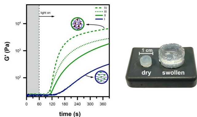
Fig. 5 a) Photo-rheology curves carried out at r.t. of formulations I, II, III and IV; and b) picture of a sample P II obtained from photopolymerisation of II, before and after swelling in water at r.t.
