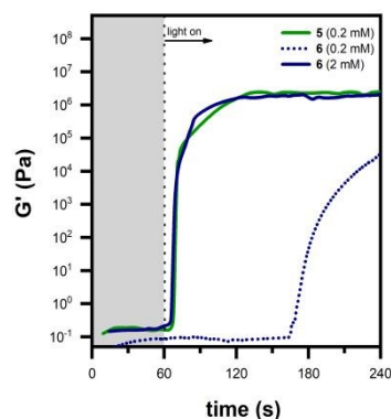
Fig. 4 Photo-rheology curves resulting from the investigation of the photopolymerization of HDDA using either equimolar PI concentration (0.2 mM) or comparing equal amount of radically cleavable groups using BAPO-Ph ( 6 ) in ten times higher concentration (2 mM) when compared to BAPO- \gamma CyD ( 5 ) (0.2 mM). The measurements were carried out at r.t., under a constant shear frequency of 1 Hz and strain amplitude of 1%, using a Hamamatsu LC8 lamp with a cut-off filter under 400 nm as light source.
