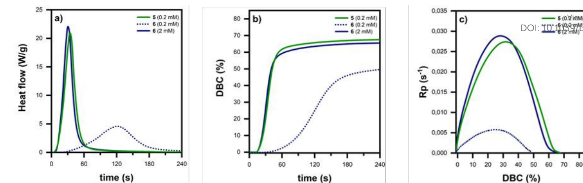
Fig. 3 a) Photo-DSC, b) double bond conversion (DBC) and c) conversion rate ( R_p ) plots resulting from the investigation of the photopolymerisation of HDDA using either equimolar PI concentration (0.2 mM) or comparing equal amounts of radically cleavable groups using BAPO ( 6 , 2mM) in ten times higher concentration than BAPO- \gamma CyD ( 5 , 0.2 mM). The experiments were carried out at r.t. under nitrogen atmosphere, using a Hamamatsu LC8 lamp with a cut-off filter under 400 nm (0.6 mW/cm 2 ) as light source.
