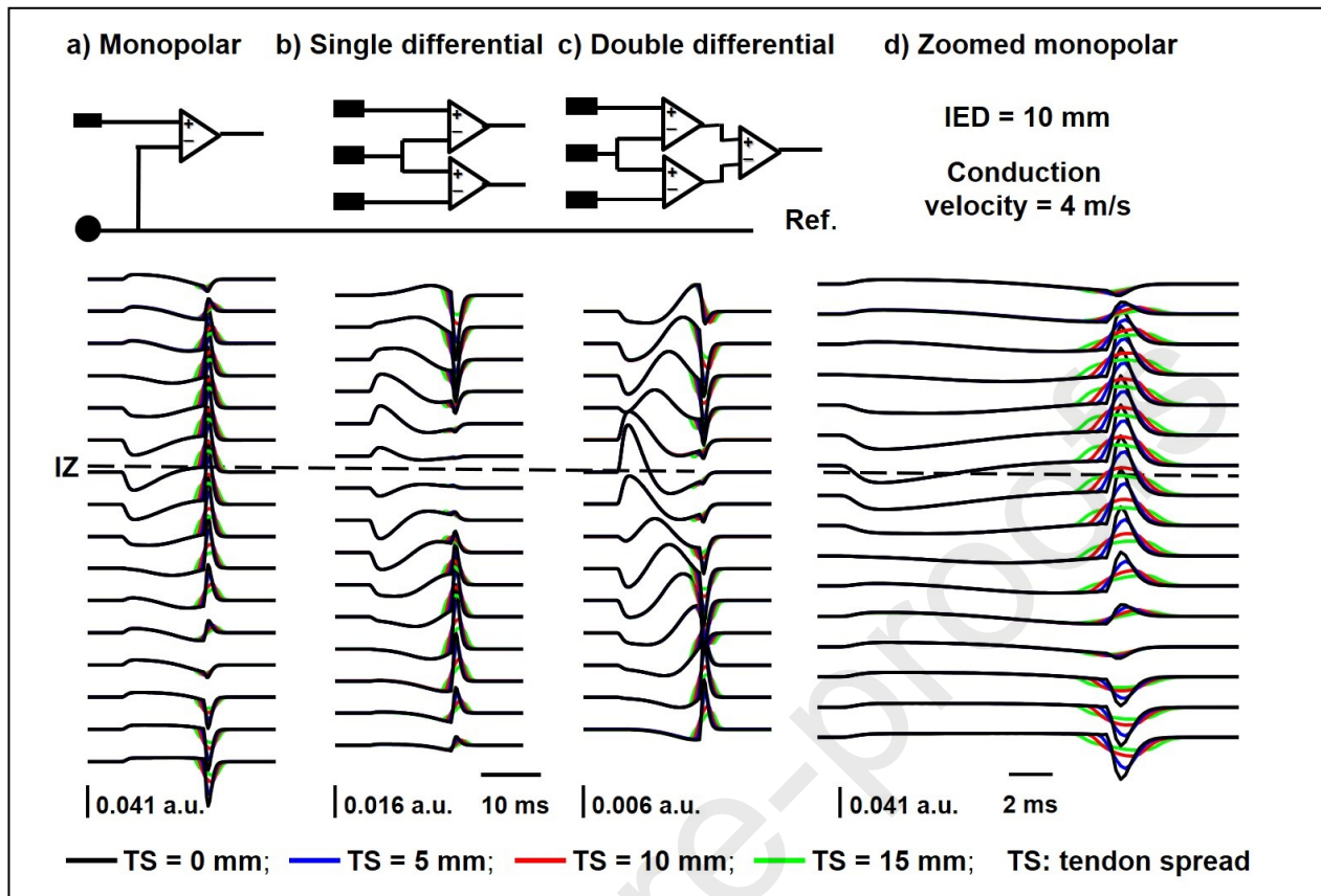
Fig. 5. Simulated action potential for a motor unit 22 mm below the skin as detected with a linear array. Except for the MU depth, all simulation parameters are the same as in Fig. 4. Example of a simulated a) monopolar, b) single differential (SD) and c) double differential (DD) MUAP showing the different impact of the end-of-fiber effect, d) time-zoomed version of the monopolar signal showing the effect of the spread of the fiber-tendon terminations. The fiber-tendon junctions have a spread (TS) indicated by the different colors. The value of the arbitrary unit of amplitude is the same as in Fig. 4. The peak-to-peak background noise value is about 0.01 a.u. (not indicated in the Figure). The SD and DD signals are near or below the noise level and therefore are barely detectable. The simulated electrodes are point-like. The a.u. units are arbitrary units that allow amplitude comparisons with respect to Fig. 4; note the different scales.
