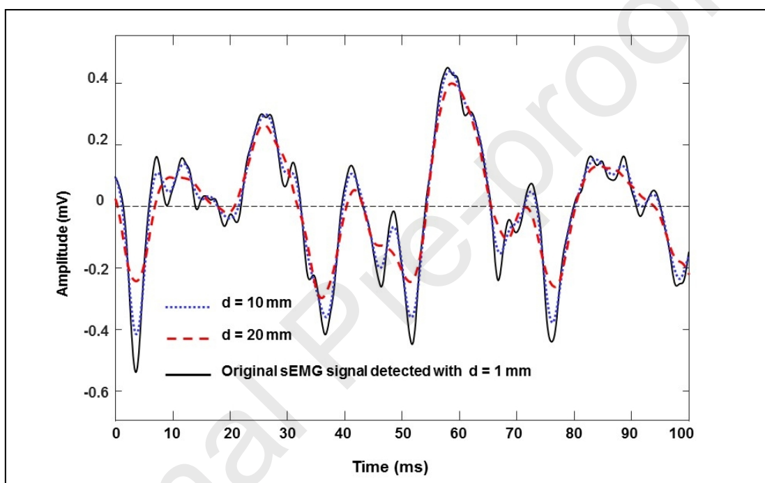
Fig. 12. Low-pass filtering effect for two different diameters of a circular electrode on a monopolar sEMG signal in time. The signal has been acquired with two pin electrodes having d = 1 \text{ mm} and has been filtered with the transfer functions depicted in Fig. 11.
