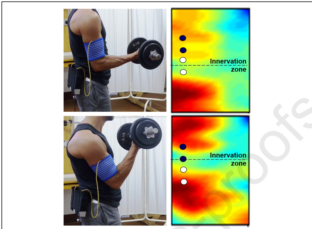
Fig. 17. Example of the effect of muscle shift under a pair of electrodes. Biceps brachii sEMG RMS map (grid of 64 electrodes, IED= 10 mm) during elbow flexion. The images are interpolated. As the muscle shortens the innervation zone shifts upward and the white electrode pair reads a progressively greater signal whereas the black electrode pair reads a progressively smaller one. These opposite changes of amplitude are not necessarily reflecting changes of muscle activity. They mostly reflect a variation of the muscle-electrode geometry (muscle shortening under the electrodes) and may be misleading and misinterpreted. The use of a sEMG map reduces the possibility of misinterpretation. Reproduced from www.robetomerletti.it .
