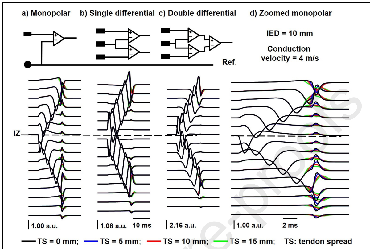
Fig. 4. Simulated action potential of a superficial motor unit as detected with a linear array. All parameters of the model are the same as for Fig. 3 except for the spread of the fiber-tendon junctions (TS). Example of simulated a) monopolar, b) single differential (SD) and c) double differential (DD) MUAP showing the different impact of the end-of-fiber effect, d) time-zoomed version of the monopolar signal showing the effect of the spread of the fiber-tendon terminations. The simulated conduction velocity is 4 m/s and the spread of the NMJs is zero. The fiber-tendon junctions have a spread indicated by the different colors. The spread of the NMJs has a very similar effect. The thickness of the skin is 1 mm and adipose layers is 1 mm. The MU has radius 3 mm, with center at a depth of 4 mm in the muscle (6 mm under the skin) and is constituted by 200 fibers parallel to the skin. The MU semi-length is 50 mm in the two directions. Note the different amplitude scales: SD and DD signal amplitudes depend on the inter-electrode distance. The simulated electrodes are point-like. The a.u. units are arbitrary units that allow amplitude comparisons; note the different scales.
