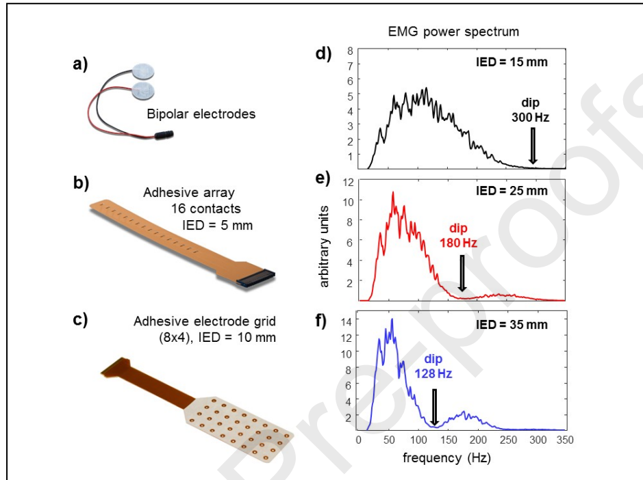
Fig. 16. Electrode types and presence of dips in experimental signals. a) Example of electrode pair, b) example of a 1D electrode array, c) example of a 32 electrode grid; d), e), f) power spectrum of three signals simultaneously obtained from a biceps brachii and from three pairs of electrodes, selected among the contacts of the linear array, centered around a central fixed point, with IED of 15 mm, 25 mm and 35 mm. The frequency of the three dips is compatible with a muscle fiber conduction velocity of 4.5 m/s. The dip for IED=15 mm is not evident because the spectrum of the specific signal is narrow. It would be more evident for a spectrum reaching 400-450 Hz. The RMS value of each signal is the square root of the area under the corresponding spectrum and is therefore affected by IED (De Luca et al., 2012). Courtesy of V. Devecchi.
