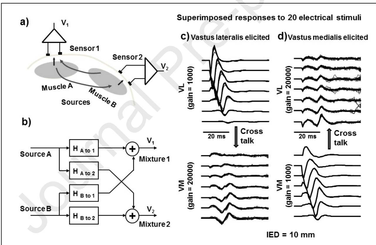
Fig. 8. Crosstalk between muscles. a) The concept of crosstalk, b) schematic model of crosstalk., c) sEMG signals detected on the vastus medialis (VM) during electrical stimulation of the vastus lateralis (VL), d) sEMG signals detected on the vastus lateralis (VL) during electrical stimulation of the vastus medialis (VM). Note the different amplifier gains and the larger crosstalk signal at the muscle-tendon region. Both electrode arrays are between the innervation zone and the muscle-tendon junction of the respective muscles. The circumferential distance between the arrays is 39 mm. H_{A\ to\ 1} is the “transfer function” (that is the filter) from the source A signal to the mixture 1 signal. Figs. 8c and d are from Fig. 1 pg 685 of (Farina et al., 2002b), with permission.
