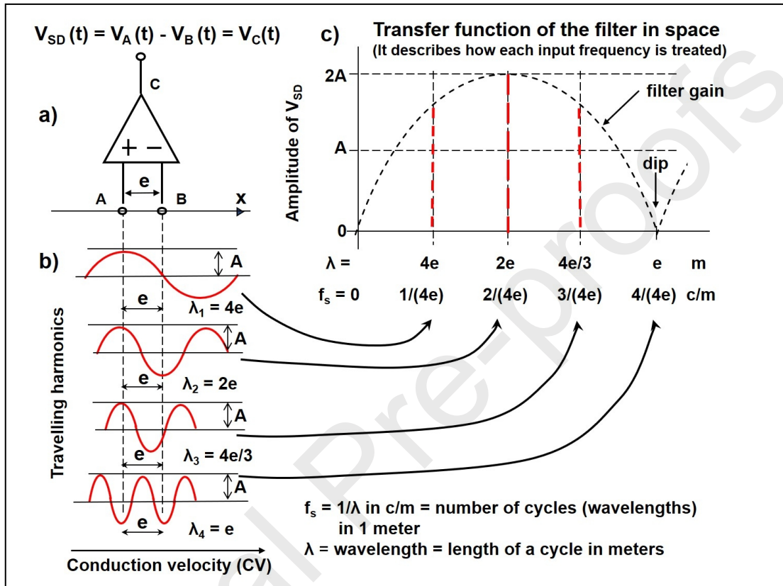
Fig. 13. Spatial filtering effect of a differential detection system. a) Differential detection system, b) four harmonics of the spatial signal distribution moving along x with velocity u . c) Amplitudes of the four harmonics observed in point C ( V_{SD} ).
