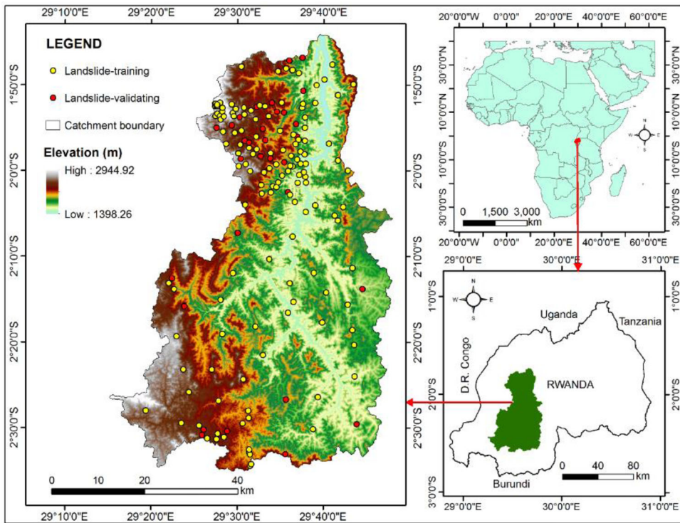
Figure 1. Location of the study area and the landslide inventory map.
