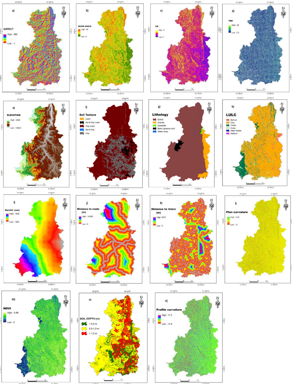
Figure 2. Landslide conditioning factors: (a) Aspect; (b) Slope angle; (c) LS, (d) TWI, (e) elevation, (f) Soil texture, (g) Lithology, (h) LULC, (i) Rainfall, (j) Distance to roads, (k) Distance to rivers/streams, (l) Plan curvature, (m) NDVI, (n) Soil depth, (o) Profile curvature.
