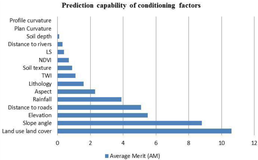
Figure 3. Prediction capability of the fifteen landslide conditioning factors in the present study.
