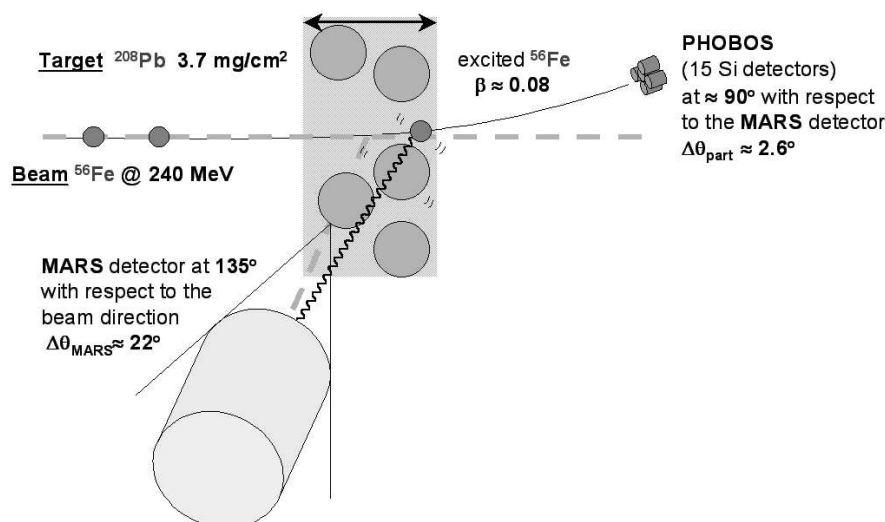
Figure 2. Setup of the in-beam experiment done at LNL with the MARS detector. A ^{56}\text{Fe} beam of 240\text{ MeV} is impinging on a 3.7\text{ mg/cm}^2 lead target. The velocity of the scattered nuclei corresponds to 8% of the light velocity. The excited ^{56}\text{Fe} is detected in the PHOBOS Si-detector array which consists of 15 single detectors with 2.6 degree opening angle. The \gamma -rays are detected in the MARS prototype which has an opening angle of 22 degree. The complete kinematics of the reaction is defined experimentally by detecting the \gamma -rays in coincidence with the excited ^{56}\text{Fe} ions.
