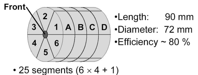
Figure 1. Schematic view of the 6x4+1 segmented HPGe MARS prototype detector.
