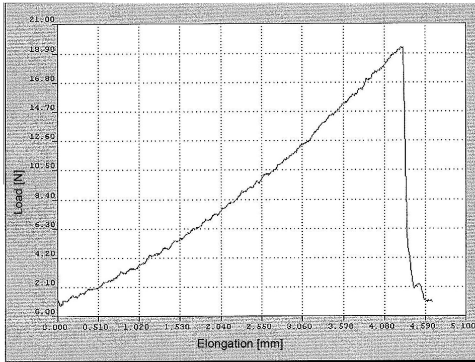
Figure 9. Elongation/load diagram for the tensile test on a Spanish Broom rope.
