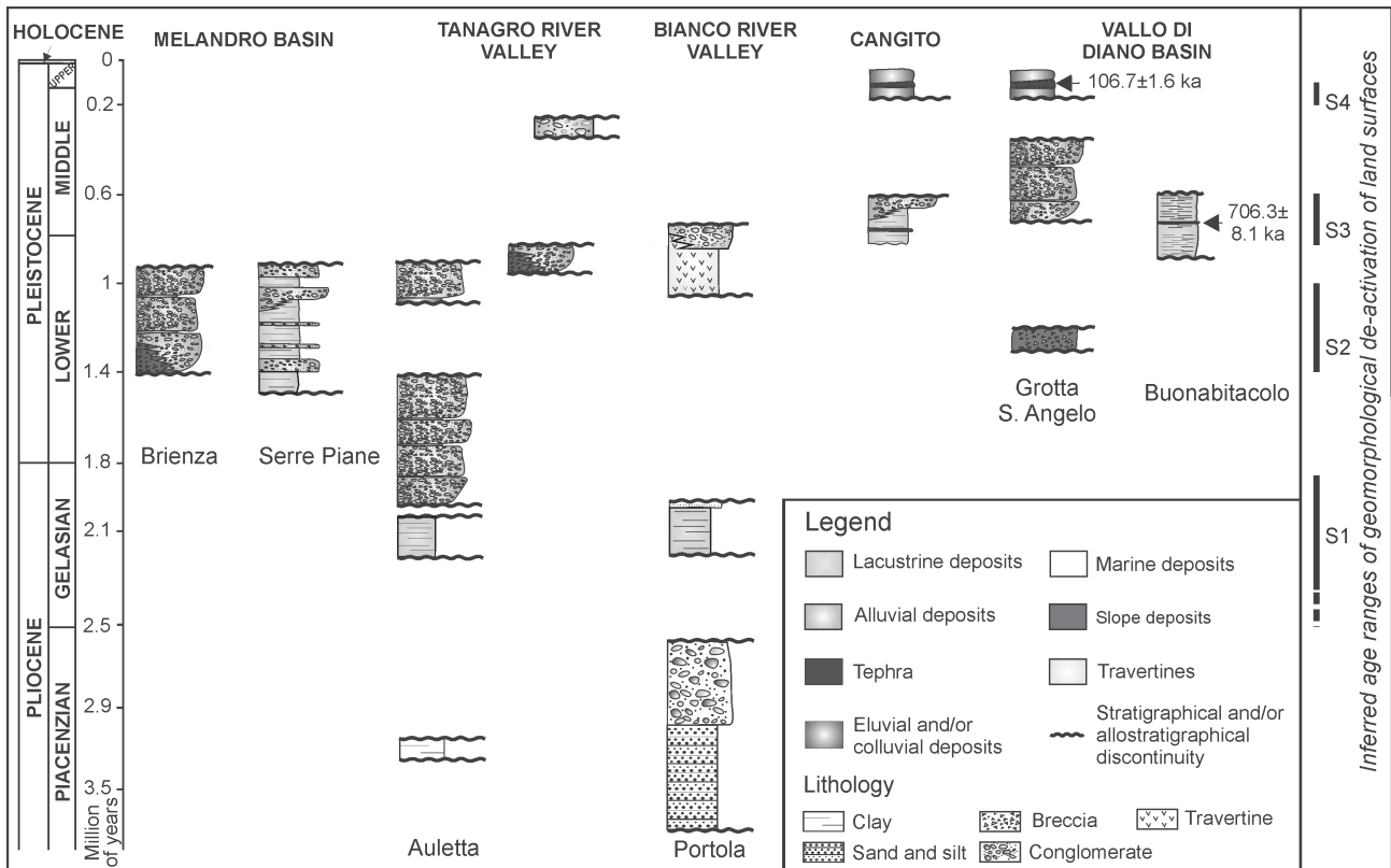
Fig. 5. Stratigraphic correlations among different logs from Vallo di Diano, Auletta and Melandro basin. The inferred ages of de-activation of the several generations of the erosional land surfaces are also shown.
