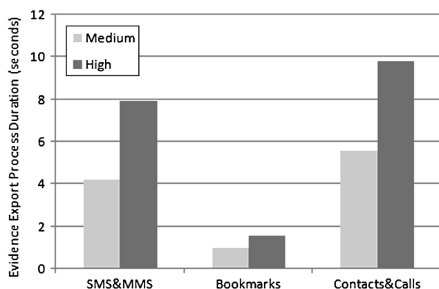
Fig. 9 – Duration, measured in seconds, of the EEP for two different amounts of Evidence to be processed.
