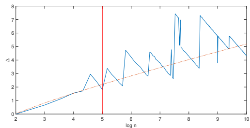
FIGURE 1. Trend of the experimental \Delta = \bar{k}_{opt} - k' (solid line) and the function \Delta = 0.5 \log n + 0.5 \log \log n - 1.467 (dashed line) over \log n .
