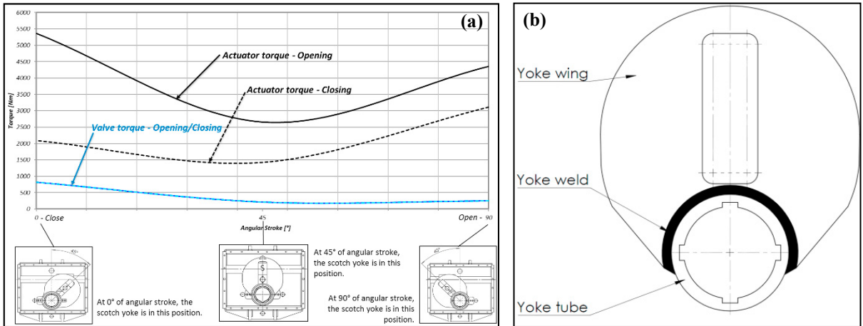
Figure 2: (a) torque comparison example graph between the valve required by the torque and that provided by the actuator, (b) scotch yoke drawing
