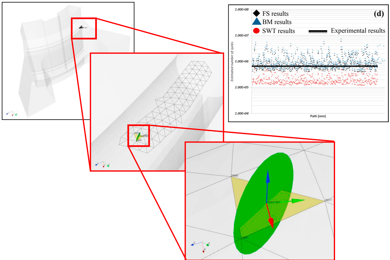
Figure 7: (a) analysed element of the weld root, (b) estimated life for a 4mm path along weld root, (c) critical element of the weld root with the critical plane, (d) fatigue life according with the three criteria examined
