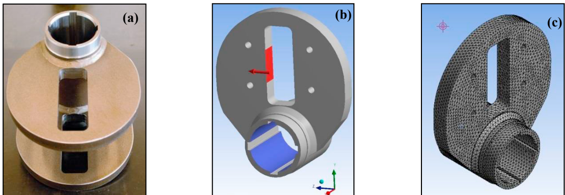
Figure 3: (a) example of scotch yoke, (b) main model, (c) FE mesh
