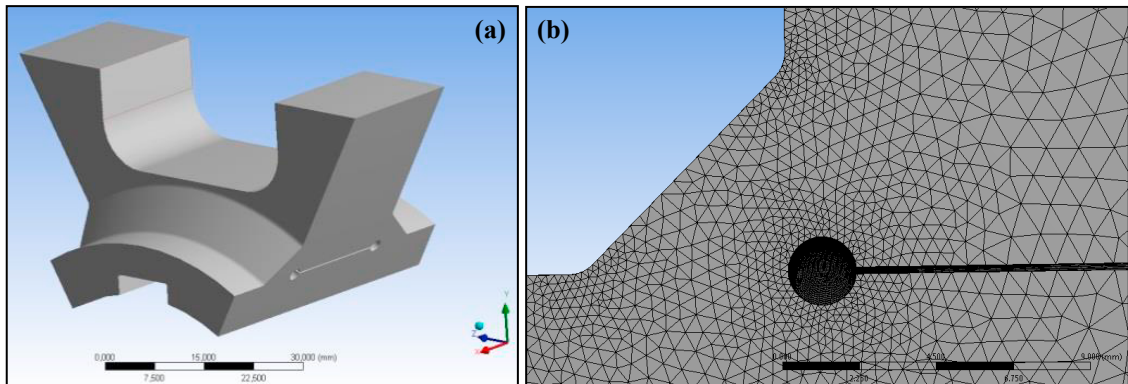
Figure 4: (a) sub-model, (b) mesh detail at weld root and weld toes
