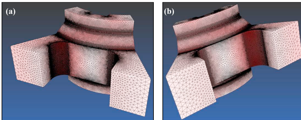
Figure 5: (a) qualitative Von Mises equivalent stress map, load case 1, (b) qualitative Von Mises equivalent stress map, load case 2. For both the pictures, the red colour highlights the highest stress
