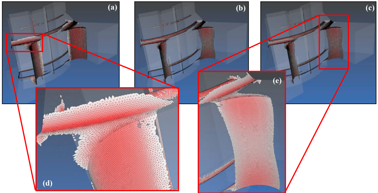
Figure 6: (a) qualitative life map obtained with Smith-Watson-Topper criterion, (b) qualitative life map obtained with Fatemi-Socie criterion, (c) qualitative life map obtained with Brown-Miller criterion, (d) critical zone enlargement from the SWT qualitative life map, (e) critical zone enlargement from the BM qualitative life map. For all the pictures reported, the red colour highlights the shortest estimated life.
