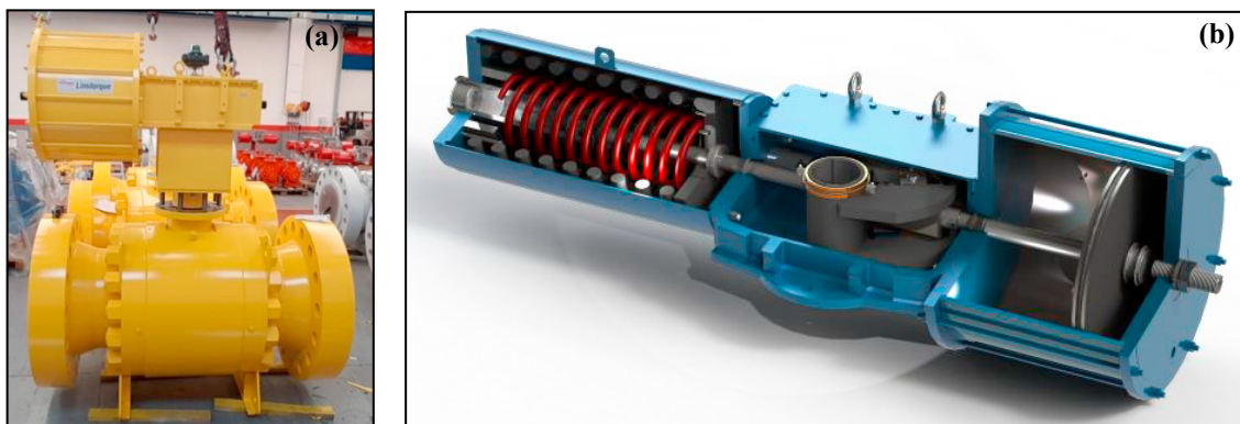
Figure 1: (a) LPS-30 actuator mounted on TMBCV Valbart valve, (b) Single acting fail close heavy-duty pneumatic actuator
