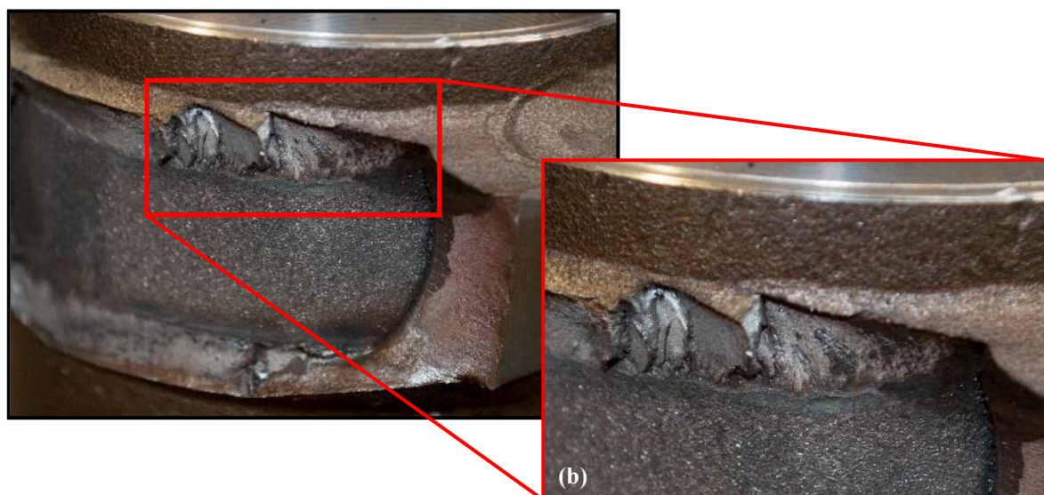
Figure 8: (a) crack of the weld in the experimental test, (b) detail of the crack planes.
