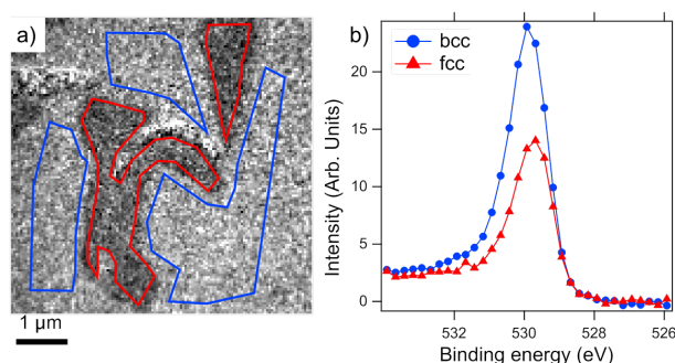
Figure 6: a) XPEEM image at the oxygen 1s core level after exposing the phase-separated alloy surface to 8.4 L \text{O}_2 . The dark (bright) regions, highlighted by the red (blue) contours, correspond to the fcc (bcc) areas. b) The XPS spectra from the bcc and fcc regions, which are marked on the XPEEM image.
