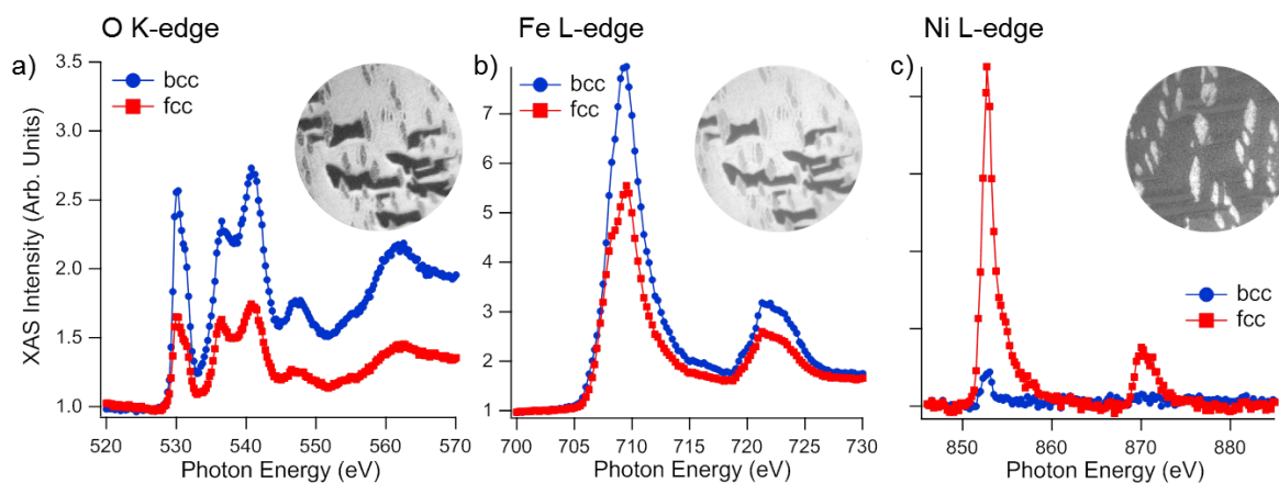
Figure 7: a) O K-edge, b) Fe L-edge, c) Ni L-edge XAS spectra from the fcc and bcc regions of a phase-separated \text{Fe}_{0.7}\text{Ni}_{0.3} film after air exposure followed by annealing at 200^\circ\text{C} in 1.10^{-6} mbar oxygen. The baseline is normalized to unity for all the spectra. The insets show the XPEEM images at the absorption thresholds (for oxygen integrated from 529 to 550 eV; for Fe and Ni at their L_3 edges) normalized pixel-by-pixel to the corresponding pre-edge intensity (senza dire image). The field of view is 5\ \mu\text{m} in all XPEEM images. The darkest regions correspond to dewetted areas, whereas the fcc regions appear as vertically elongated islands. Ni spectra is taken from a different region on the same surface.
