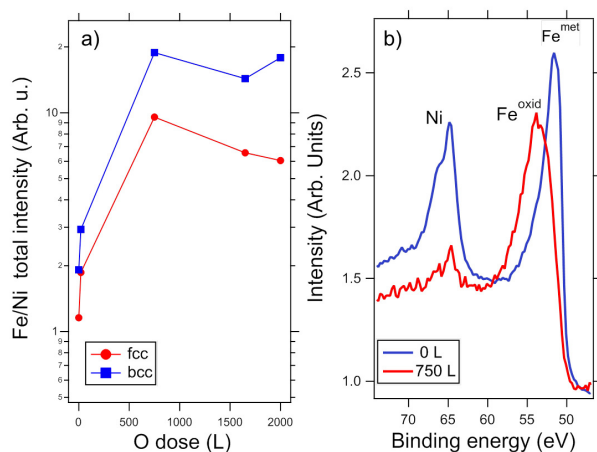
Figure 2: a) Evolution of the Fe 3p and Ni 3p core-level intensity ratio as a function of O 2 exposure. b) Comparison of the XPS spectra at the two core levels acquired at 0 L and 750 L oxygen exposure. Photon energy is 250 eV.
