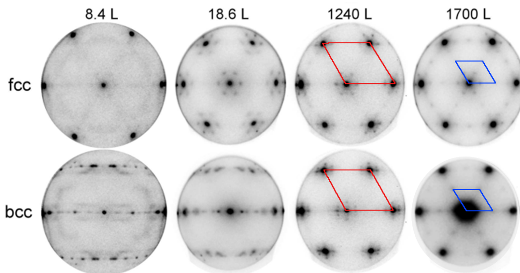
Figure 5: \mu -LEED patterns as a function of oxygen dose for the fcc (top row) and bcc (bottom row) phases present in the phase-separated alloy surface. Electron energy is 45 eV. The unit cell for the FeO and Fe 3 O 4 phases are indicated in the image (red and blue lines, respectively); substrate [1 \bar{1} 0] direction is along the horizontal axis.
