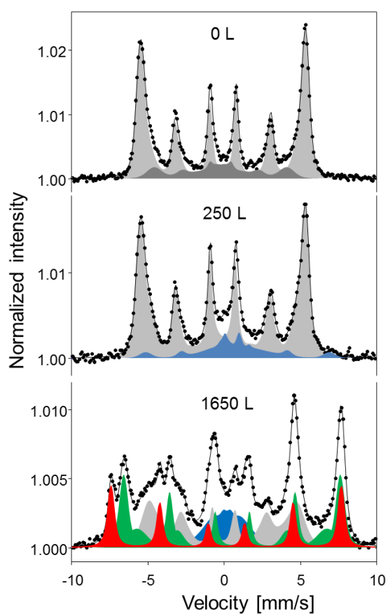
Figure 4: CEMS spectra from the \text{Fe}_{0.7}\text{Ni}_{0.3} film are shown for varying oxygen dose. The measurement averages over both fcc and bcc phases of the phase-separated alloy film. The spectral components are color-coded: light gray – metallic FeNi; red – tetrahedral site in spinel; green – octahedral site in spinel; blue – non-specific oxide components. For the top spectrum of the pristine film the decomposition into bcc-FeNi (light gray) and fcc-FeNi is shown
