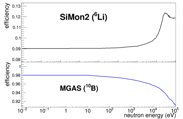
Fig. 4. (Top panel) SiMon2 efficiency for the detection of products from the ^6\text{Li}(n, t)\alpha reaction. (Bottom panel) Efficiency for detecting the products of the ^{10}\text{B}(n, \alpha)^7\text{Li} reaction in the MGAS detector.
