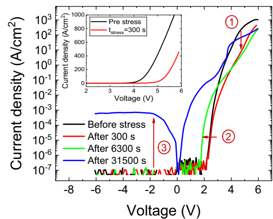
Fig. 4. Changes in the I–V curves measured during constant current stress ( J_{\text{stress}} = 0.7 \text{ kA/cm}^2 ) carried out at different stress times. We can identify three main phenomena: the decrease in the current probably due to p-type activation process (1), the increase in the current at the low forward voltage region (2) and the increase in the reverse bias leakage current (3). Inset: I–V characteristics (linear graph) measured before stress and after 300 s at 0.7 \text{ kA/cm}^2 .
