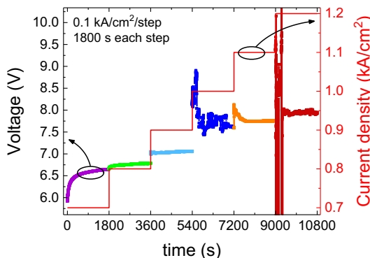
Fig. 2. Result of a step-stress measurement: the current density is increased by 0.1 \text{ kA/cm}^2 every 1800 s starting from 0.7 \text{ kA/cm}^2 until failure is reached ( 1.2 \text{ kA/cm}^2 ).
