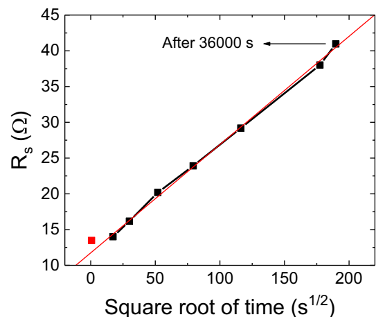
Fig. 8. Relation between the increase in the series resistance and the square root of stress time.
