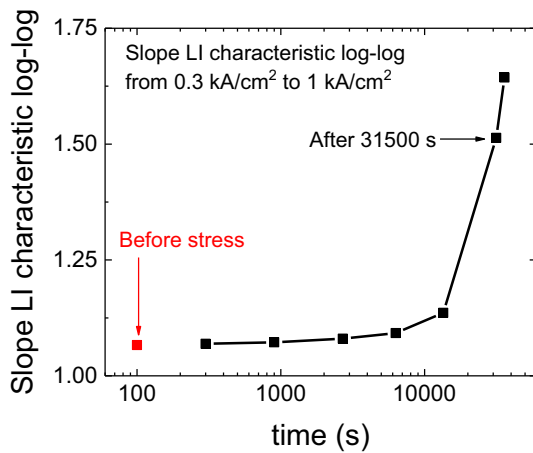
Fig. 6. Changes in the slope of the L-I characteristics (log-log graph) measured during the stress.
