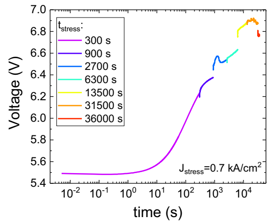
Fig. 3. Temporal variation of the voltage during constant current stress. The diode is stressed at 0.7 \text{ kA/cm}^2 for 36,000 s.
