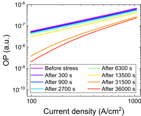
Fig. 5. L-I characteristics measured before stress and after each step of the stress at nominal current density (0.7 kA/cm 2 ).
