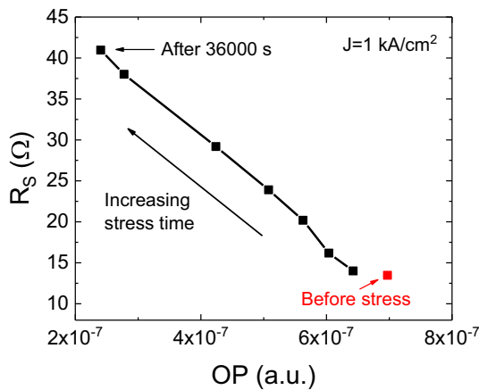
Fig. 7. Relation between the decrease in the optical power measured at 1 kA/cm 2 and the increase in the series resistance during the stress.
