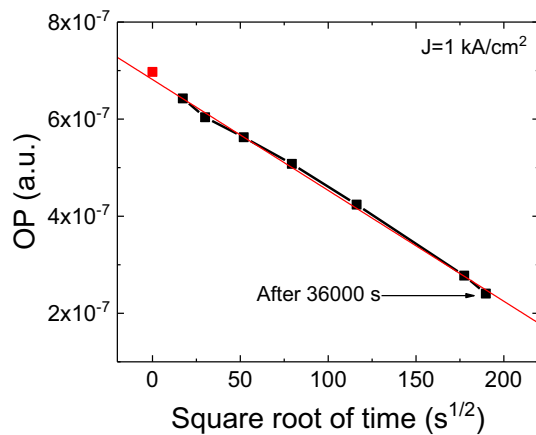
Fig. 9. Relation between the variation of the optical power measured at 1 kA/cm 2 and the square root of stress time.
