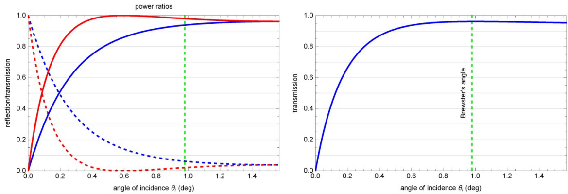
Fig.6. (a) Reflection and Transmittance coefficient for s- and p- polarization light; (b) Transmittance for un-polarization light
