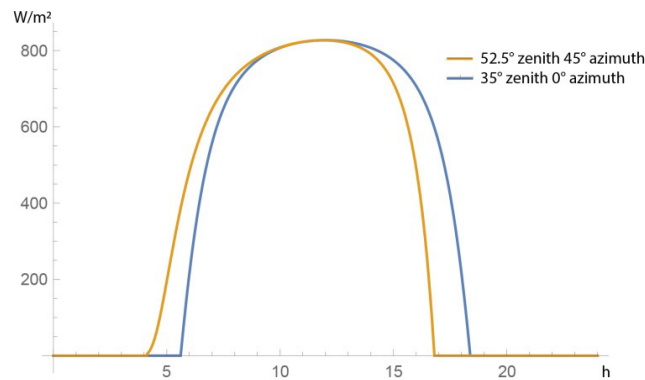
Fig.7. Direct radiation transmitted on 21 June in panels with fourth cases study: tilt and exposure ( 52.5^\circ and 45^\circ azimuth) and with “standard” position ( 35^\circ zenith and 0^\circ azimuth)
