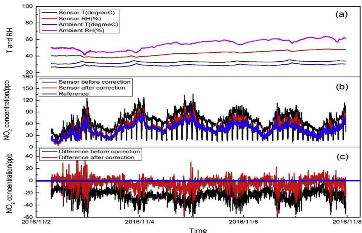
Fig. 1. Sensor performance relating to changes in temperature, RH, and drift. Example of a low-cost \text{NO}_2 electrochemical sensor with an \text{O}_3 filter. Test is displaying responses to changes in temperature, relative humidity, and drift over time (Ning, 2018).
