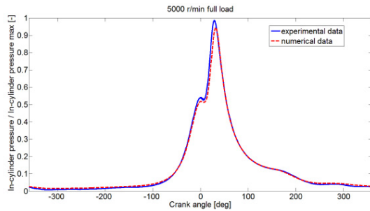
Fig. 1.: Comparison between experimental and numerical in-cylinder pressure
