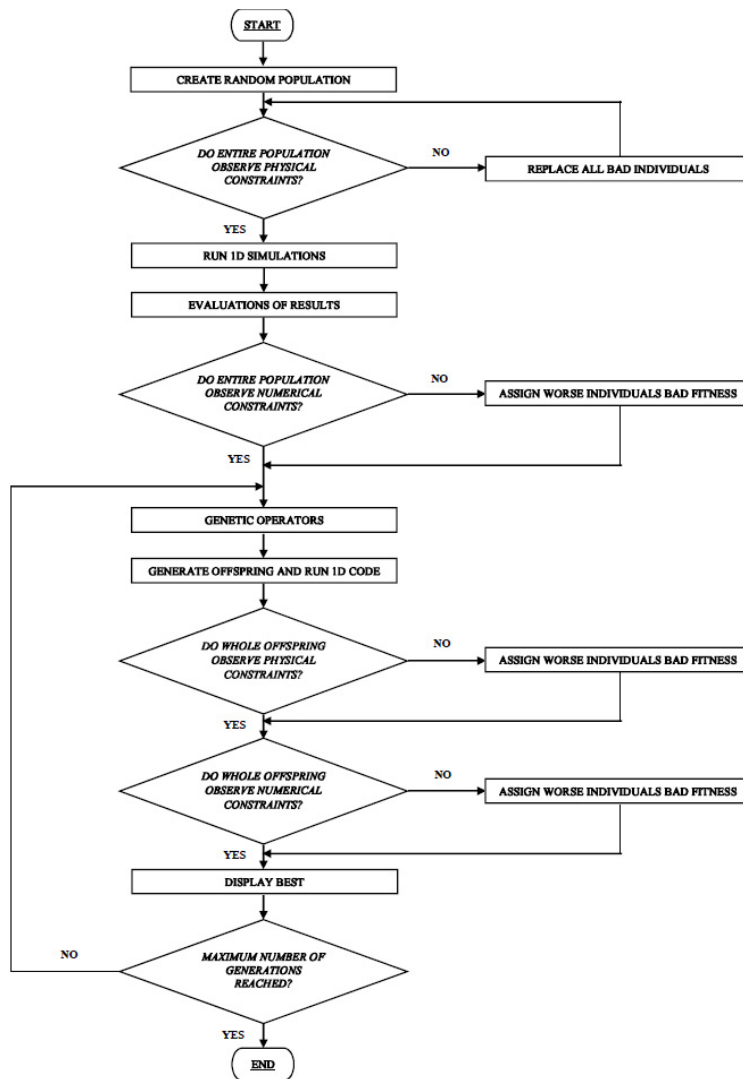
Fig. 5.: Flowchart of the optimization tool
