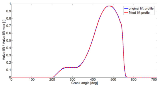
Fig. 3.: Comparison between original and fitted lift profile for 1500 r/min
