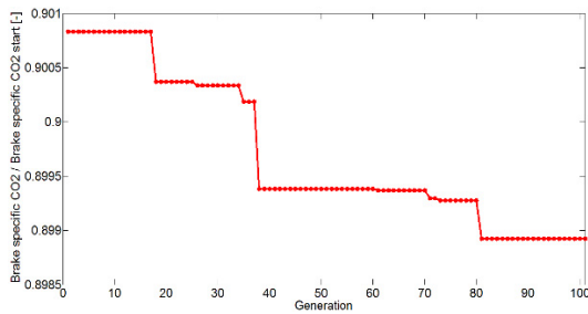
Fig. 6.: Reduction of CO_2 vs. number of generations
