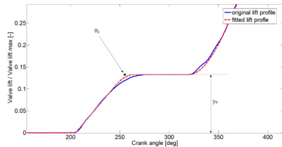
Fig. 4.: Start angle of pre-lift and pre-lift high explanation
