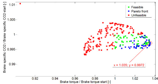
Fig. 9.: Objective space for 1500 r/min full load
