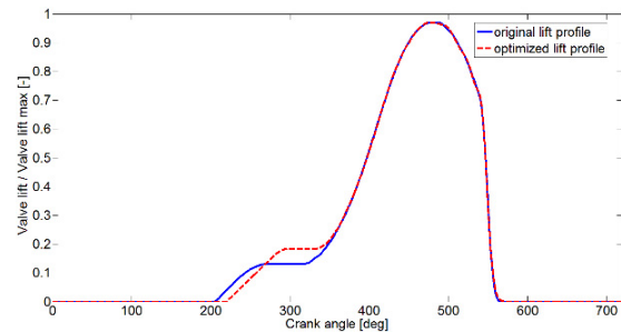
Fig. 10.: Optimized lift profile at 1500 r/min full load
