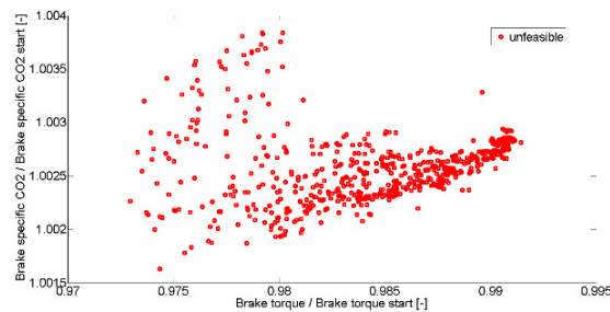
Fig. 8.: Objective space for 5000 r/min full load
