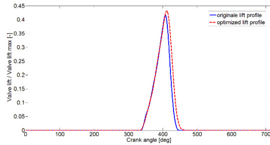
Fig. 7.: Optimized lift profile at 2000 r/min
