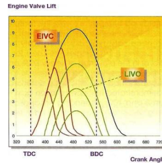
Fig. 2.: Achievable lift profiles with MultiAir VVA system [7]
