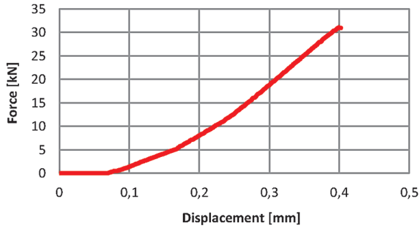
Fig. 3. Force-Displacement curve at specimen 031 (laminated CF_OHC)
