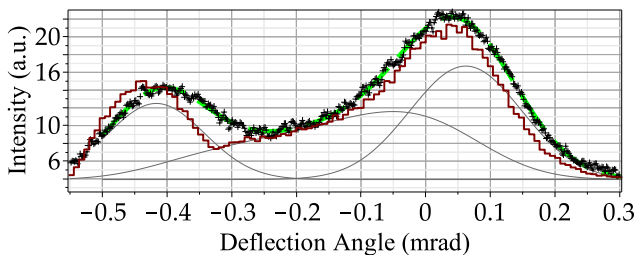
FIG. 4. (Color online) Example of the fit to 3.35 GeV channeling data at 0 mrad crystal angle. Plot symbols and lines have the same meaning as in Fig. 3. For this example, channeling efficiency is 22%, surface transmission, 62% and the dechanneling length, 38 \mu\text{m} .
