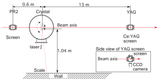
FIG. 1. Top view layout of the experiment.
