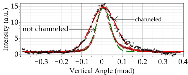
FIG. 7. (Color online) Vertical profiles of channeled (black +) and not-channeled (brown \times ) beam at 6.3 GeV together with Gaussian fits (dashed lines). The 1\text{-}\sigma width of the channeled particles is 60\ \mu\text{rad} , while the 1\text{-}\sigma width of the not-channeled particles is 35\ \mu\text{rad} , consistent with 39\ \mu\text{rad} from the multiple-scattering formula[38]. The data sets are intensity-normalized to each other.
