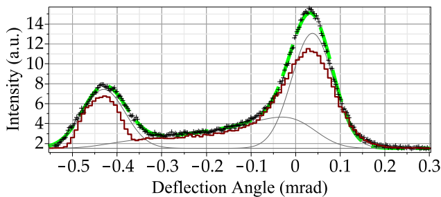
FIG. 3. (Color online) Example of the fit to 6.3 GeV channeling data at 0 mrad crystal angle. The dashed line (green) is the fitted function, the crosses are the measured intensity. The solid dark-grey lines represent the individual contributions to the fit (Gaussian peaks, dechanneling tail and constant background). For this example, channeling efficiency is 23.8%, surface transmission, 55% and the dechanneling length, 33 \mu\text{m} . The maroon histogram is from DYNECHARM++ simulations, see text.
