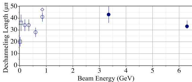
FIG. 6. (Color online) Published data for the dechanneling length of electrons in Si crystals. The two open boxes indicate data for (110) planar channeling in straight crystals[30]; the open circles, (110) straight crystal[7]; the open diamond, (111) straight crystal [8] Table 1); the solid circles are this work, (111) bent crystal.
