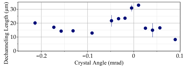
FIG. 5. (Color online) Dechanneling length vs. crystal angle, 6.3 GeV. Error bars reflect the scattering of the underlying data from several frames; the data points at -0.05 mrad and +0.045 mrad have larger uncertainty due to beam jitter.
