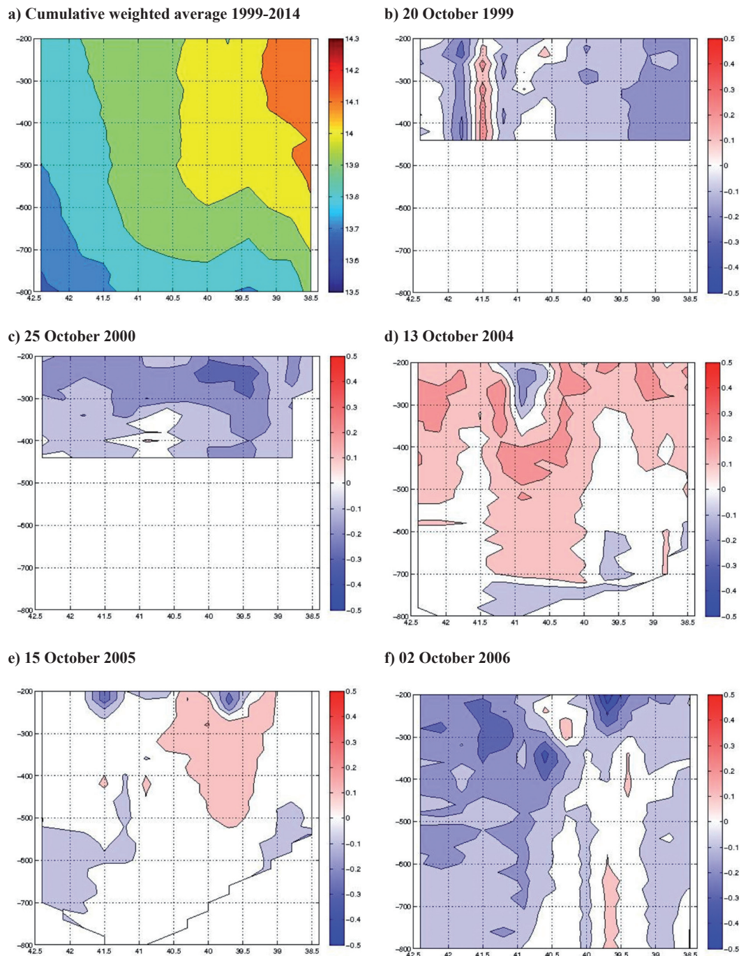
Fig. 6: (a) cumulative weighted average built from the entire dataset of 2054 XBT profiles between 42.5°N and 38.5°N in the range 200-800 m depth for the period 1999-2014. (b) to (k) anomalies recorded during representative single cruises in the period September-December with respect to a). Values in color bar are in °C.
