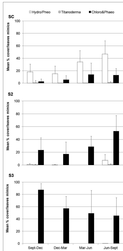
Fig. 5: Trend of settlement (algal cover) of the main macroalgal taxa in the artificial leaves of P. oceanica in the period Sept 2009 - Sept. 2010 along the gradient, in the south side of Castello Aragonese. Bars represent standard deviations.
