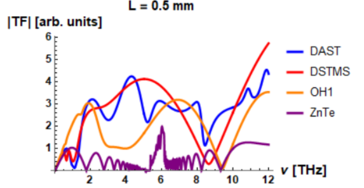
Figure 1: Modulus of the transfer function TF(L, \omega) (in arbitrary units) for the crystals ZnTe, DAST, DSTMS and OH1 in the range 0 – 12 THz. The crystals are considered to have the same length L = 0.5 mm
