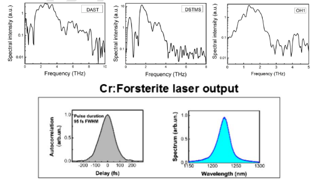
Figure 2: Top: Terahertz spectrum emitted by DAST, DSTMS and OH1 retrieved by first order autocorrelation in a THz Michelson interferometer taken from Ref. [16]. Bottom: the Cr: forsterite laser output taken from Ref. [7].
