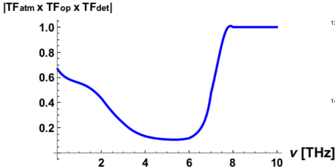
Figure 4: Modulus of the reconstructed function TF_{atm} \times TF_{op} \times TF_{det} relative to the pump retrieval of Fig. 3. This is the necessary correction to the transfer function, as expressed by Eq. (7), which allows to take into account both for the losses due to the THz propagation in air and those due to the finite acceptance and chromatic effects related to the optical components.
