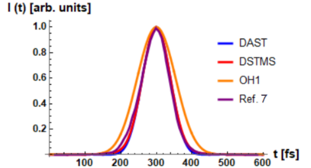
Figure 3: The comparison between the pump envelope deduced from the autocorrelation measurement of Ref. [7] (purple curve, FWHM 95 fs) and the temporal envelopes of the pump for the different crystals, reconstructed starting from the THz spectra reported in Fig. 2.
