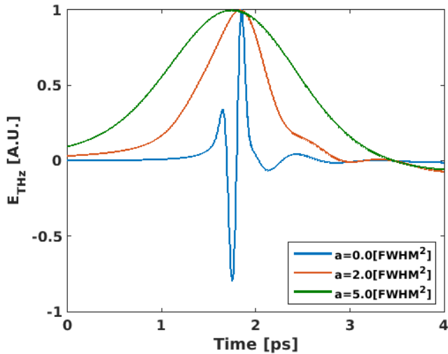
Figure 5: THz field produced by OR in DSTMS crystal L = 0.5 mm with a pump of \lambda = 1250 nm and FWHM = 100 fs for different value of the chirp coefficient a . The amplitudes have been normalized to obtain the same peak value for easier reading.
