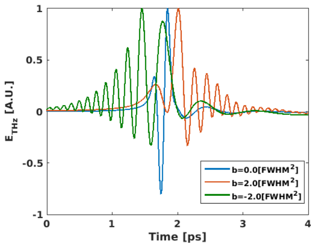
Figure 6: THz field produced by OR in DSTMS crystal L = 0.5 mm with a pump of \lambda = 1250 nm and FWHM = 100 fs for different value of the third order dispersion coefficient b . The amplitudes have been normalized to obtain the same peak value for easier reading.
