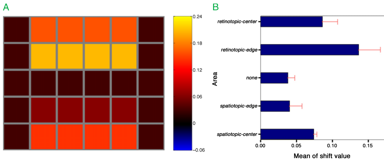
Figure 7. (A) Comparing different regions of the MAE topographic map after a saccade. Five different areas including retinotopic edge and central lines, spatiotopic edge and central lines, and the non-adapted area are contrasted based on their MAS values. (B) MAS mean values in different regions. In order to compare the critical areas of the map, the rightmost and leftmost columns of the test area were discarded and the mean value of MAS across each horizontal band was determined. The error bars represent one standard error of mean.
