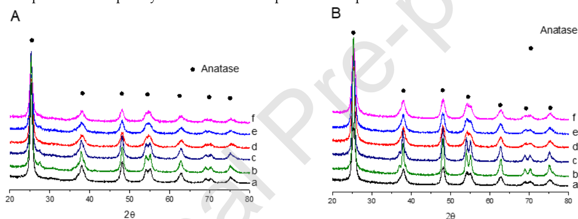
Figure 2. Diffractograms of bare and Co- \text{TiO}_2 prepared via (A) solution and (B) hydrothermal methods; a) bare \text{TiO}_2 , b) Co(0.25%)- \text{TiO}_2 , c) Co(0.5%)- \text{TiO}_2 , d) Co(1%)- \text{TiO}_2 , e) Co(3%)- \text{TiO}_2 , f) Co(5%)- \text{TiO}_2
