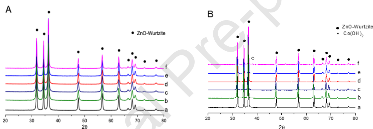
Figure 1. Diffractograms of bare and Co-ZnO prepared via (A) solution and (B) hydrothermal methods, a) pristine ZnO, b) Co(0.25%)-ZnO, c) Co(0.5%)-ZnO, d) Co(1%)-ZnO, e) Co(3%)-ZnO, f) Co(5%)-ZnO
