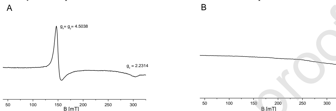
Figure 4. EPR spectra of A) Co(1%)-ZnO via solution synthesis and B) Co(1%)-TiO 2 via solution synthesis.
