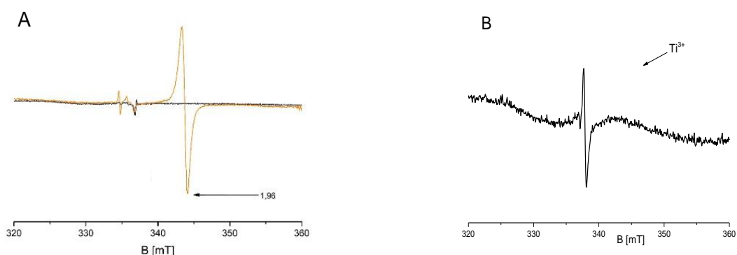
Figure 5. Comparison of bare and cobalt doped Oxides. A) bare ZnO (orange) and Co(1%)-ZnO (black) via solution synthesis; B) bare TiO 2 (orange) and Co(1%)-TiO 2 (Black) via solution synthesis.
