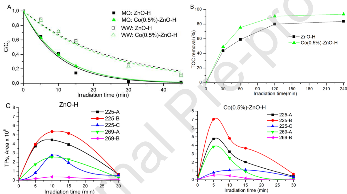
Figure 8. A) Ketoprofen degradation over time (20 mg/L) under UVA irradiation in the presence of (1000 mg/L) Co(0.5%)-ZnO-H and ZnO-H in Milli-Q water (MQ) and in real wastewater sample (WW). B) TOC removal in during ketoprofen degradation in the presence of ZnO-H and Co(0.5%)-ZnO-H in Milli-Q water. C) Ketoprofen transformation products over time observed in the presence of ZnO-H and Co(0.5%)-ZnO-H.
