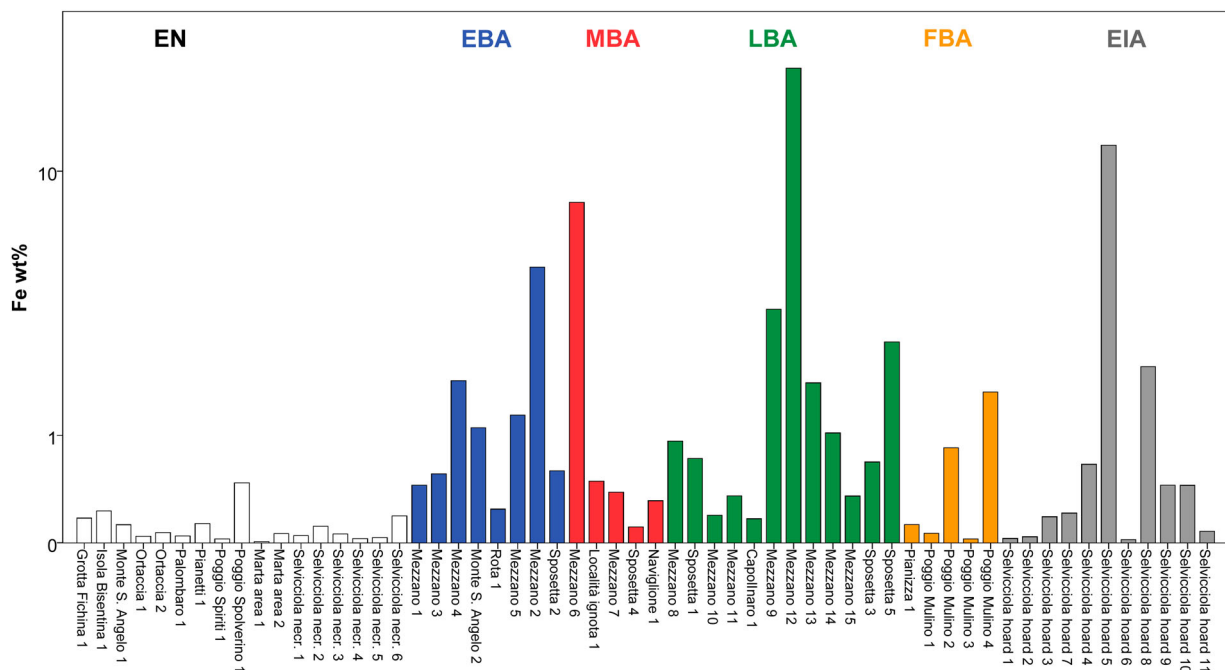
Figure 10. Bar-chart of the Fe mean concentration for all artefacts; a pseudo-logarithmic transform y = \text{sign}(x) \cdot \log(1 + \text{abs}(x)) is applied to the vertical axis to improve readability of low values; white, blue, red, green, orange and grey bars refer to Eneolithic, Early Bronze Age, Middle Bronze Age, Late Bronze Age, Final Bronze Age and Early Iron Age, respectively.
