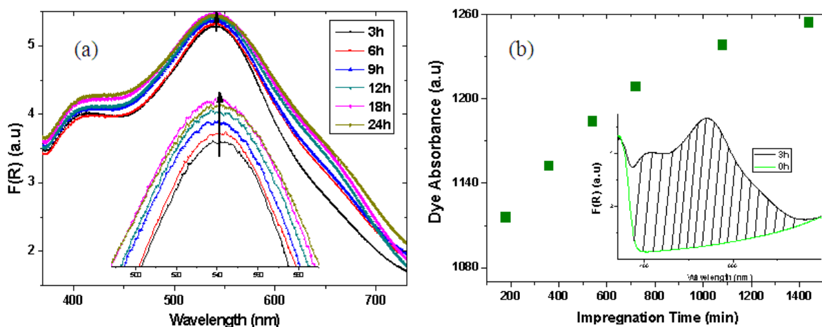
Figure 3: (a) Absorption spectra of photoanodes after dye impregnation for different time periods, (b) Area between F(R) curves after and before dye incubation (shown in inset only for 3h to have clear view).
