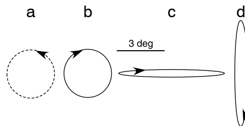
Figure 3 . Scale drawing showing that when a spot's clockwise circular orbit ( b ) lay on a counterclockwise background orbit ( a , dashed line) that was out of phase with its horizontal component, it was judged as matching a wide ellipse ( c ) with an aspect ratio of 14:1. When the background was out of phase with its vertical component, it was judged as matching a tall ellipse ( d ) with an aspect ratio of 7.5:1. Drawing is to scale. Scale bar shows 3 deg of visual angle.
