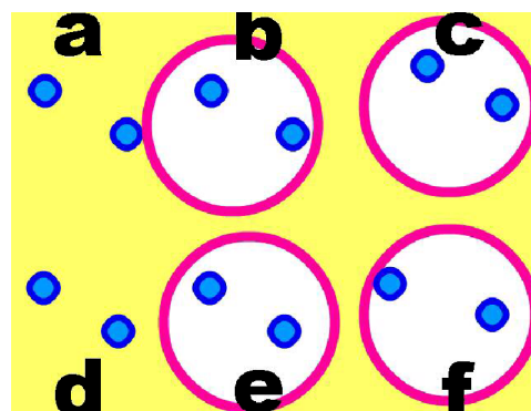
Movie 5. Summary. Pairs of dots rotating clockwise (a and d). Clockwise surround (b) makes left orbit look larger (c). Counterclockwise surround (e) makes dots appear to move up and down or left and right (f). Click on the image to view the movie.
