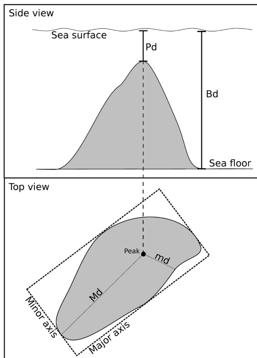
Fig. 1: Main physiographic characteristics of seamounts.
