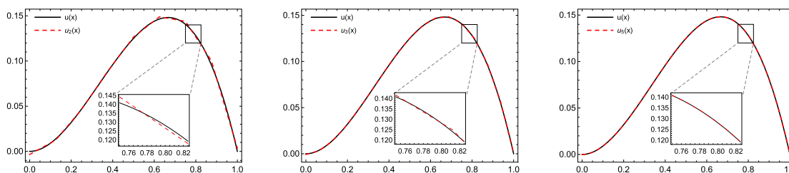
Fig. 6 The comparison between approximate and exact solutions of Example 5.1 using system I.
