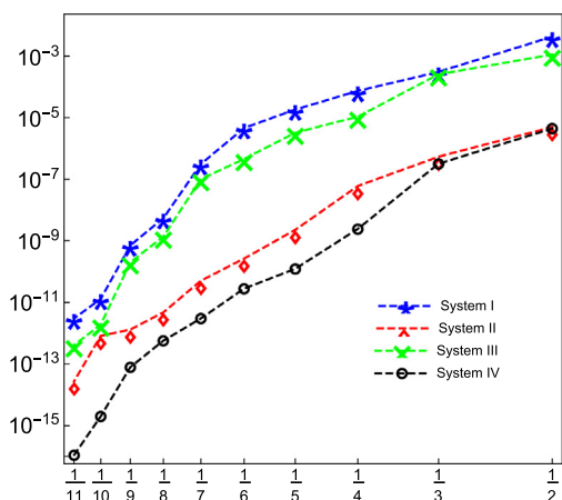
Fig. 10 Behavior of convergence rate for Examples 5.1 given in the log-log scale plot.
