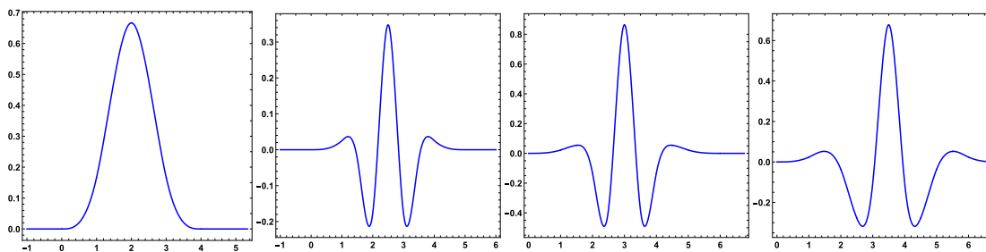
Fig. 5 The B-spline B_4(x) and the corresponding quasi-affine generators via the OEP.
