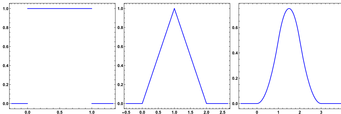
Fig. 1 The refinable functions, B_m , for m = 1, 2, 3 .
