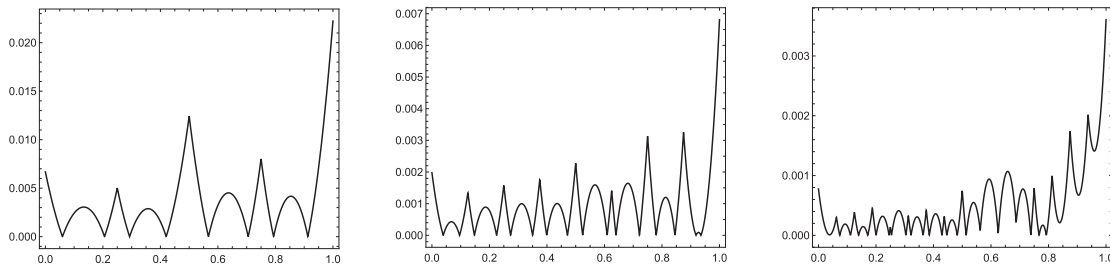
Fig. 15 The graphs of E_n(x) , n = 1, 2, 3 , respectively, of Example 5.3 using System I.
