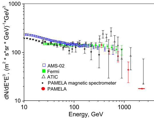
Figure 6: The obtained electron-positron spectrum in compare with direct measurements.
