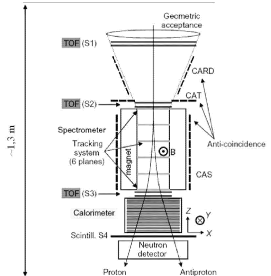
Figure 1: The PAMELA instrument.
