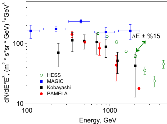
Figure 7: The obtained electron-positron spectrum in compare with ground-based measurements.
