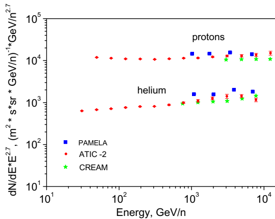
Figure 9: The obtained proton and helium spectra in compare with ATIC-2 and CREAM results.
