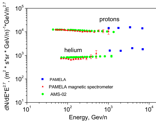
Figure 8: The obtained proton and helium spectra in compare with AMS-02 and magnetic spectrometer PAMELA results.
