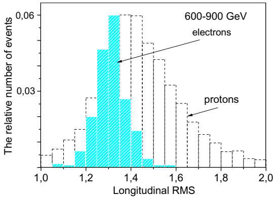
Figure 3: The longitudinal RMS distribution. The simulation data.
