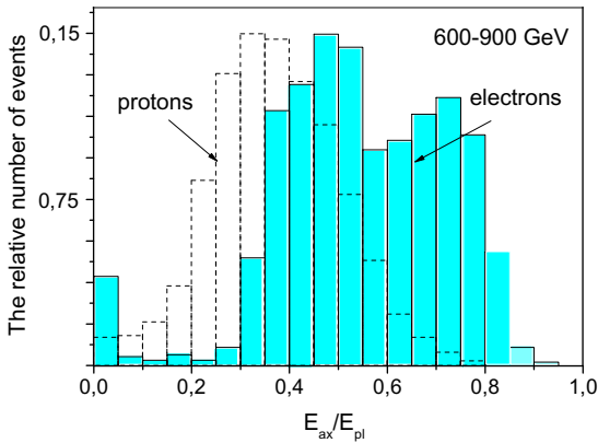
Figure 4: The distribution of ratio E_{ax}/E_{pl} , where E_{ax} - the energy release along the shower axis for plane 2, E_{pl} - the energy release in plane 2. The simulation data.
