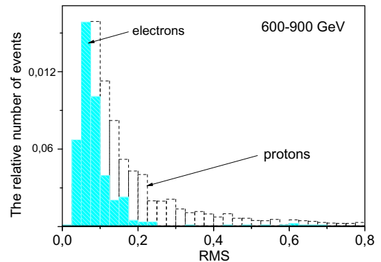
Figure 2: The distribution of RMS deviations for the second subset of the calorimeter planes. The simulation data.
