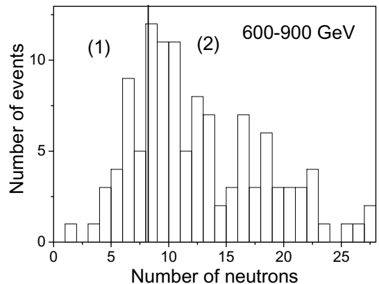
Figure 5: The neutron number distributions. The experimental data.
