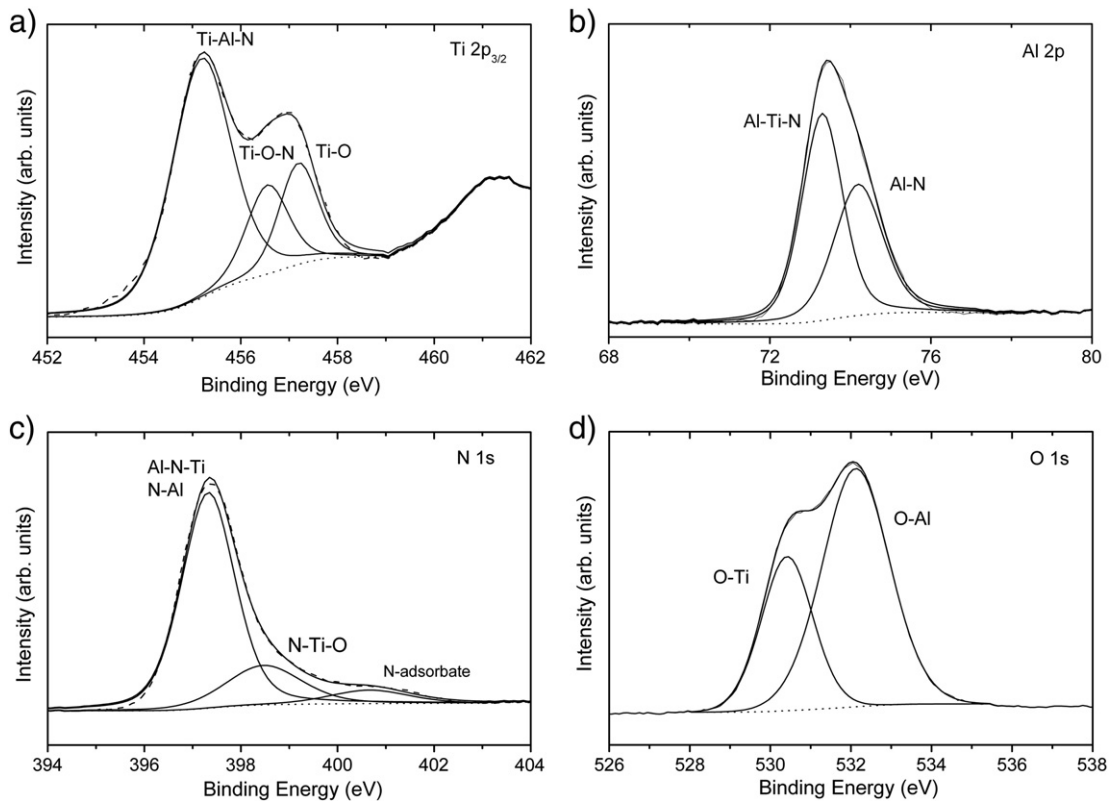
Fig. 4. XPS peak fittings of (a) Ti 2p, (b) Al 2p, (c) N 1s and (d) O 1s regions for a TiAlN/AlN-n representative coating.
