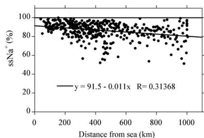
Fig. 2. Percentage contribution of \text{ssNa}^+ with respect to total \text{Na}^+ reported as a function of distance from the sea.
