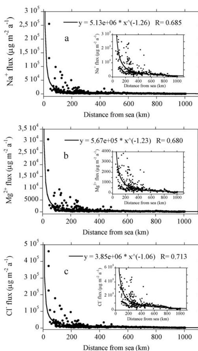
Fig. 3. \text{Na}^+ (a), \text{Mg}^{2+} (b) and \text{Cl}^- (c) depositional fluxes as a function of distance from the sea. Smaller plots inside the panels show the same plot at lower y scale.
