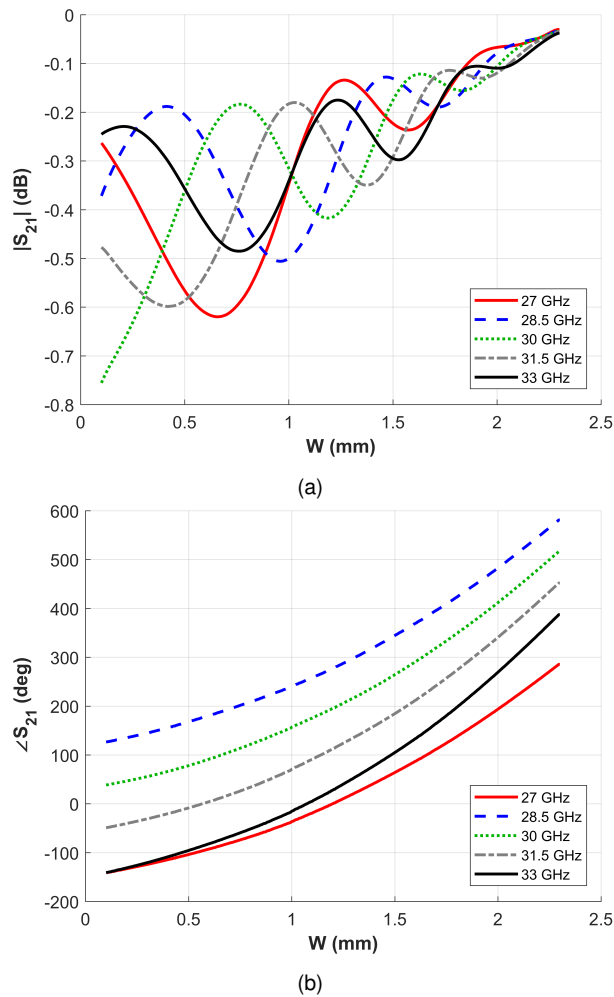
FIGURE 3: Simulated transmission coefficient as a function of W for different frequencies: (a) Amplitude |S_{21}| ; (b) Phase \angle S_{21} .
