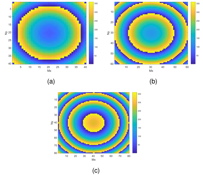
FIGURE 6: Required phase distribution for the three designed TA configurations: (a) 40x40 elements TA; (b) 60x60 elements TA; (c) 80x80 elements TA.
